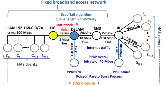
Fig. 1: Network architecture used in ns-3.
