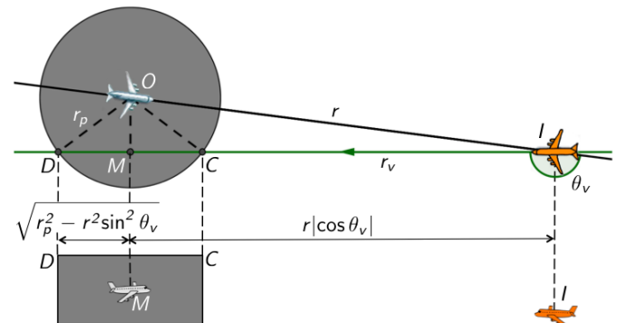
Figure 1: Reduction to a 2-dimensional encounter
