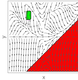
Figure 3: Safety verification problem from [37].
