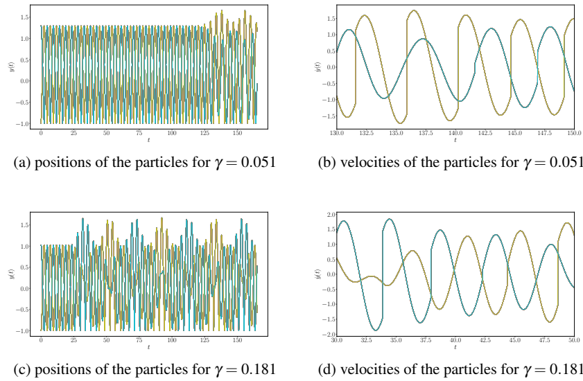
Fig. 21: Time integration of the periodic solutions for the out-of-phase mode with pattern I_1 = \{2k + 1\}_{k=0,\dots,49}, I_2 = \{2k\}_{k=0,\dots,49}
