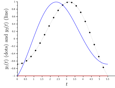
(b) Particle oscillations for \gamma = 0.2, T = 11
