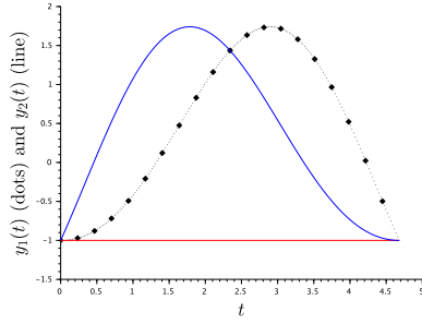
(a) Particle oscillations for \gamma = 0.2, T = 4\pi(1 + 4\gamma)^{-1/2}
