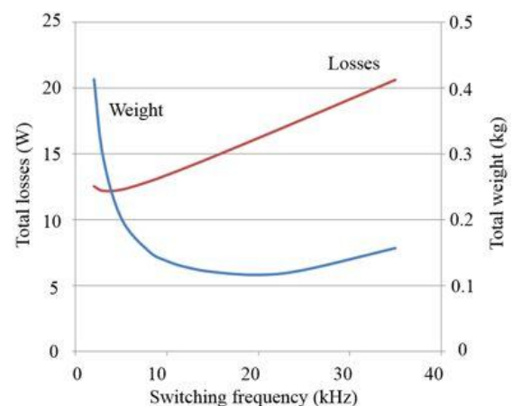
Fig. 1. Evolution of weight and losses of a 1kW converter vs switching frequency.
