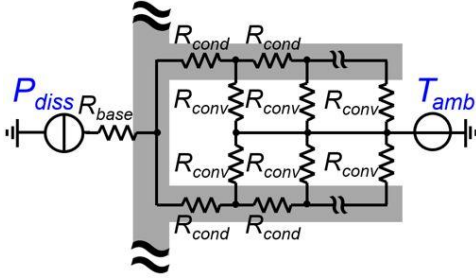
Fig. 4. Modeling of the fins temperature gradient effects by a network of y thermal resistance modules.
