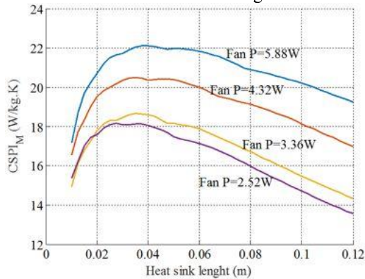
Fig. 8. Calculated heatsink performance index CSPI_M for different aluminum heatsink lengths and different 40x40mm fans. Curves are shown for optimal k and number of fins. High length values cause high pressure drop in the heatsink channels which reduces the heat extraction capability. CSPI_M is low for short heat sinks due to the fan weight.
