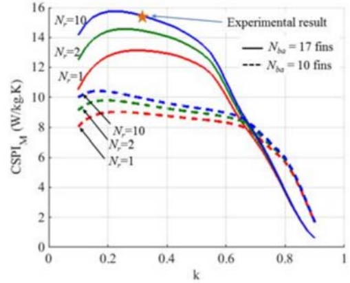
Fig. 6. Calculated heatsink performance index CSPI_M for different fin widths (represented by k ), number of fins ( N_{ba} ) and number of elements ( N_r ) used to model the heatsink. Measured value in a customized heat sink is marked by a star. Great error in heatsink resistance may exist for thin fins if heat sink is modeled by only one element in the resistance network.
