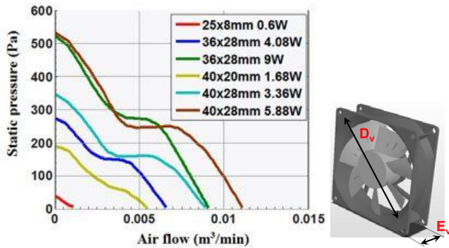
Fig. 2. Hydraulic characteristics of different axial fans having different power and dimensions.
