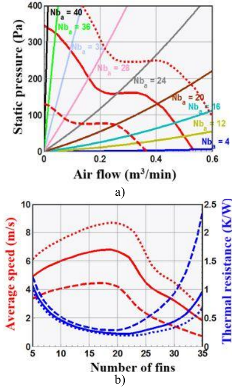
Fig. 5. Design of heat sinks with forced convection for heat sinks of same external dimensions and with different number of fins and for three different fans. a) static pressure versus air flow rate characteristic of fans and b) evolution of the mean speed between fins and the thermal resistance function of the number of fins.
