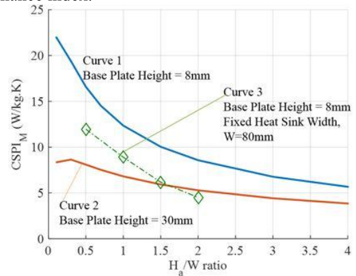
Fig. 9. Calculated aluminum heatsink performance index CSPI_M for different height/width ratios. Curve 1 and 2 have no fixed width but fixed front surface (6400mm 2 ), fixed fan characteristic and base plate height of 8 and 30mm respectively. Curve 3 has fixed base plate and different fin heights having different number of rows containing 2 side-by-side fans. Optimal cooling system for this fixed base plate configuration has 1 row of 2 side-by-side fans (fin height is half the base plate width).
