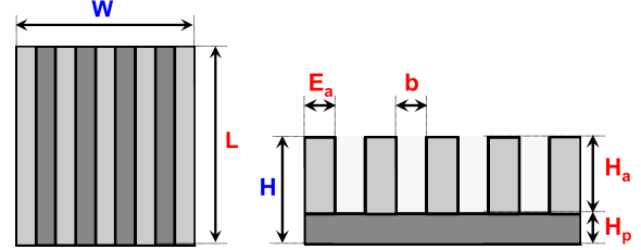
Fig. 3. Extruded heatsink dimensions; a) top view; b) front view.
