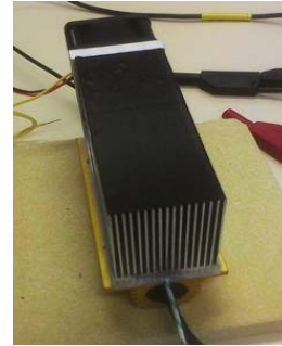
Fig. 7. Manufactured heat sink used to verify the accuracy on thermal resistance model having 10 elements in the resistance network. Weight = 0.286kg and thermal resistance = 0.23K/W.
