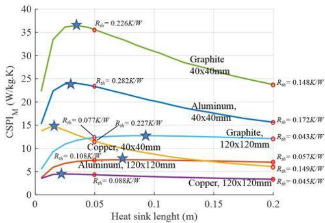
Fig. 10. Calculated heatsink performance index CSPI_M for different heatsink lengths, materials and front sizes: Case 1 - 40x40mm (using 1 fan); Case 2 - 120x120mm (using 3 rows of 3 side-by-side fans). Curves are shown for optimal k and number of fins. Aluminum heat sinks have higher performance index than copper ones. Graphite have the highest performance index but it is around 10 times more expensive than aluminum. Maximum performance index for each case is marked with a star and the thermal resistance for some points are marked with circles. Note that each considered heat sink is entirely made of a unique material.
