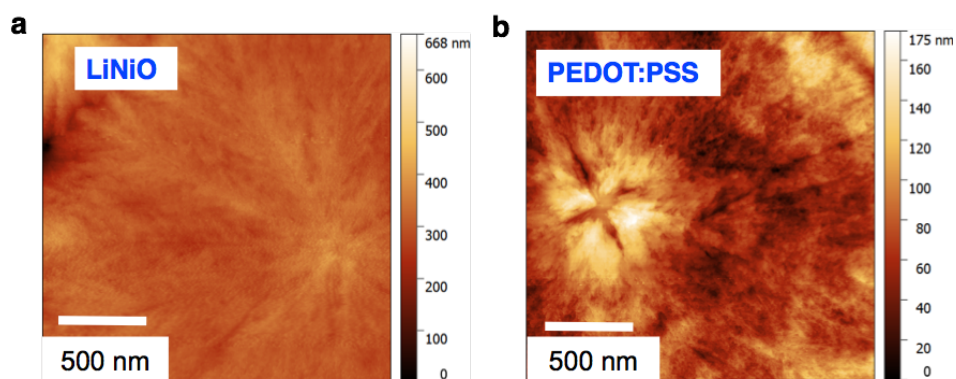
Figure S1. AFM images of MAPbI 3 grown on LiNiO and PEDOT:PSS (a, b).
