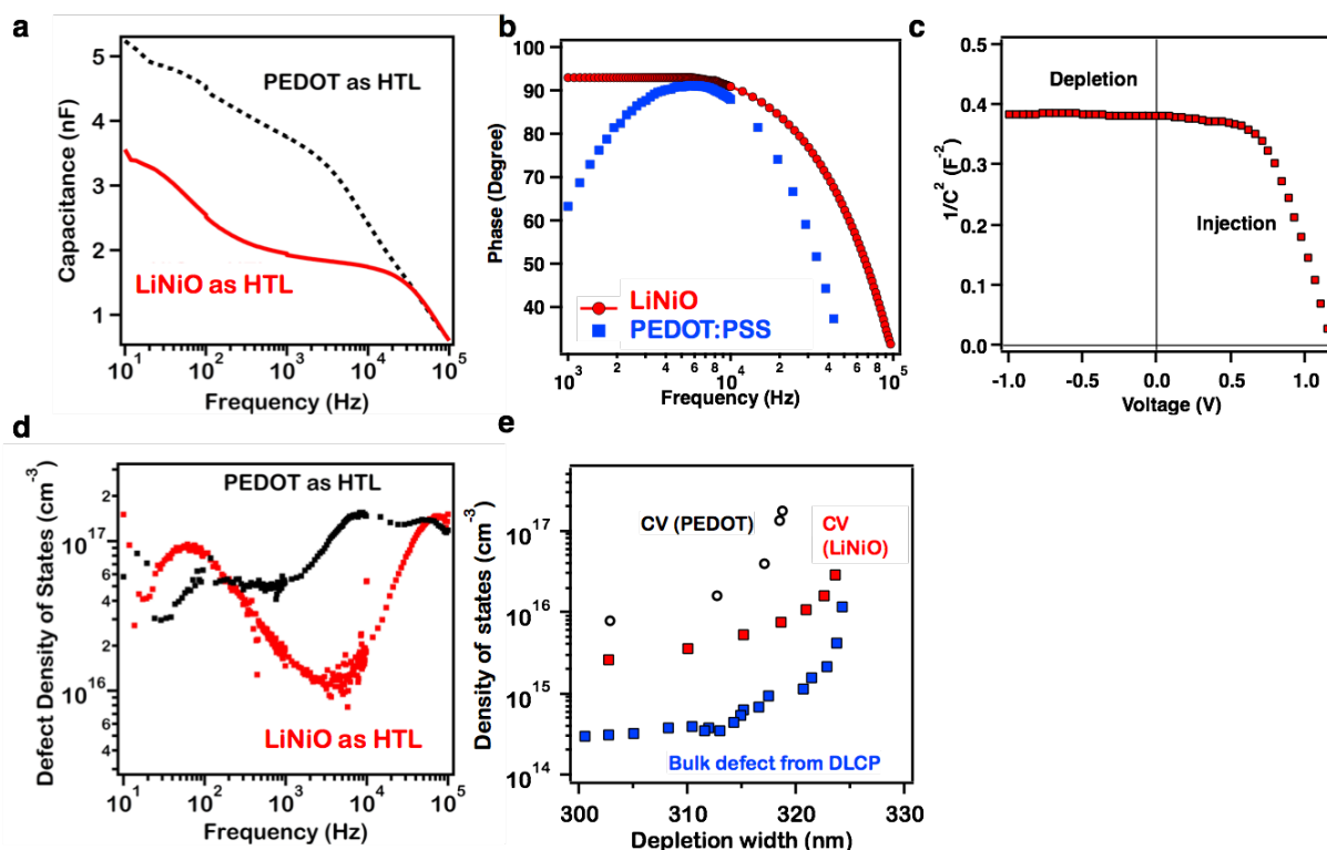
Figure S6 Impedance spectroscopy characterization for MAPbI 3 device using LiNiO and PEDOT:PSS as HTL. a , capacitance as a function of frequency spectrum. b , phase angle as a function of frequency. c , capacitance-voltage curve plotted according to Mott-Schottky relation for the LiNiO device. d , defect density of states calculated from a . e , defect density of states measured by capacitance-voltage curve near the depletion region edge for LiNiO and PEDOT:PSS. The bulk defect density is obtained by measuring the non-linear capacitance using drive level capacitance profiling method.
