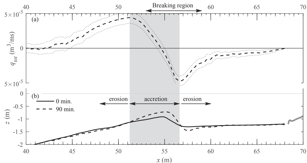
Fig. 5. (a) Total transport during the experiment ( t = 0-90 min) obtained through Eq. (4), mean values (dashed) \pm 95\% confidence interval (dotted) over all experimental repeats; (b) Initial (solid) and final (dashed) bed profile. The grey shading marks the region of net accretion.
