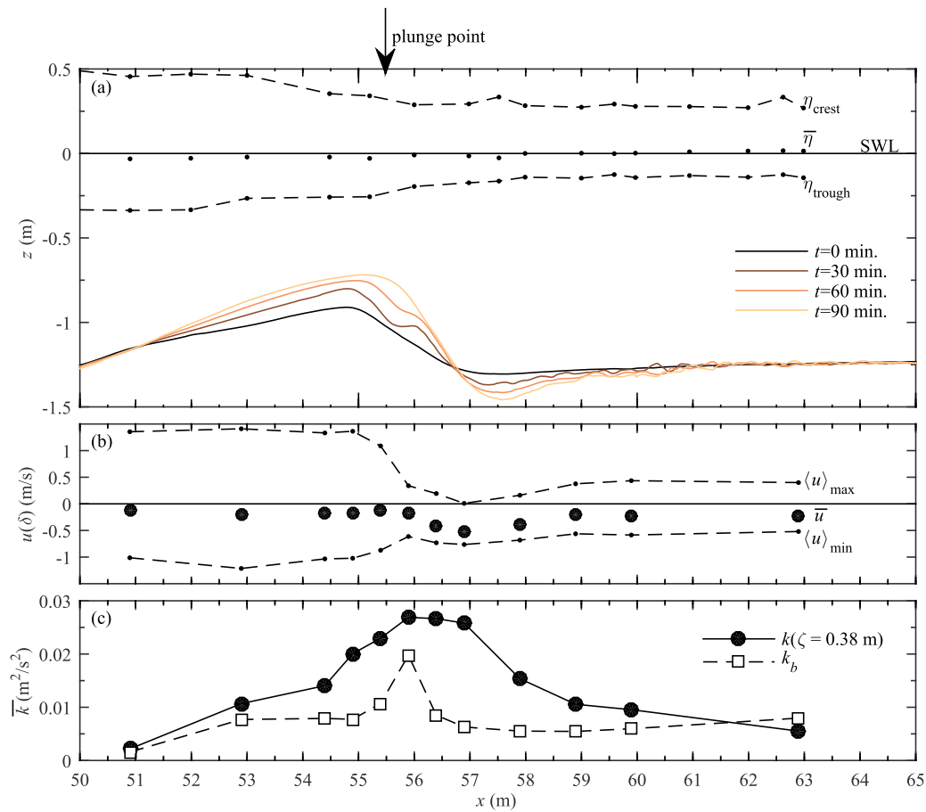
Fig. 4. (a) Bed profile evolution (solid lines, with each line representing the mean value over all experimental days), and water levels for t = 0-15 min (dots and dashed lines depict time-averaged and envelope, respectively); (b) ACVP-measured horizontal velocity at the WBL overshoot elevation \zeta = \delta , for t = 0-90 min, time-averaged (circles) and maximum phase-averaged onshore and offshore velocity (dots and dashed line); (c) Time-averaged turbulent kinetic energy over the experiment ( t = 0-90 min) at outer-flow elevation \zeta = 0.38 m (measured with ADV, solid line + circles) and inside the WBL (measured with ACVP, dashed line + squares).
