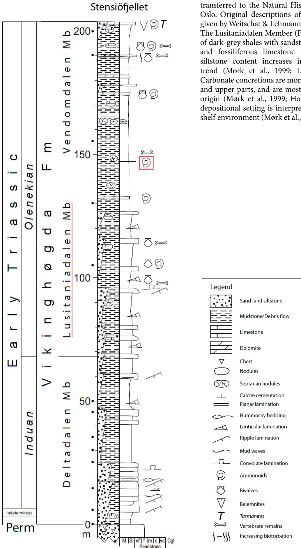
Figure 3. Stratigraphic log section of the Vikinghøgda Formation at Stensiøfjellet. The red square represents the concretion horizon from which the studied fauna most likely came (modified from Vigran et al., 2014, figs. 18 & 38a).
