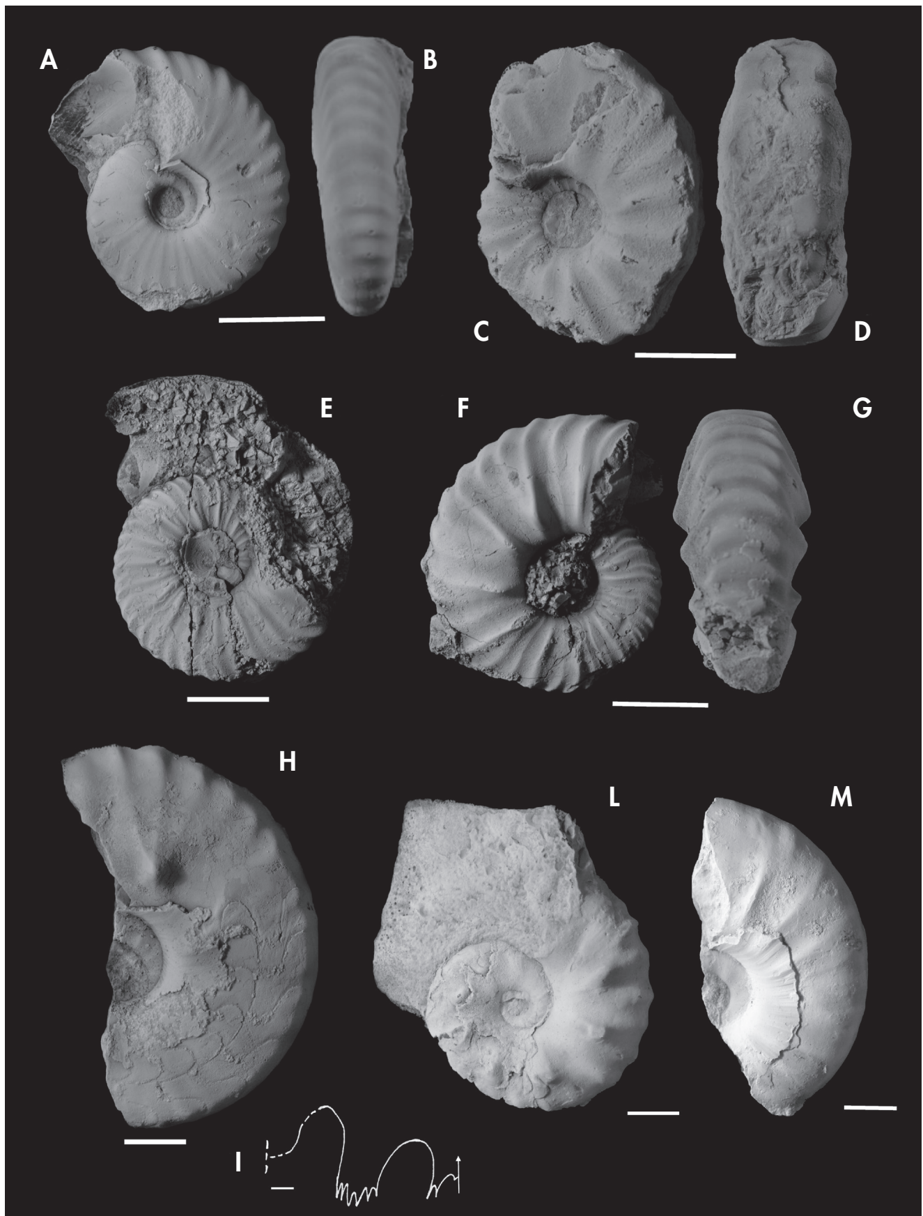
Figure 5. (A–E) Wasatchites spp. indet. Specimens are classified as juvenile/immature stages of Wasatchites because they bear either faint tubercles or none at all: (A–B) PMO 228.012, (C–D) PMO 228.000, (E) PMO 228.011; (F–I) Wasatchites tridentinus Spath, 1934. The not fully mature individual (F–G) still has defined ribbing, which becomes weaker on adult stage (H–I): (F–G) PMO 228.009, (H–I) PMO 228.010. Scale bar for the suture lines = 25 mm; (L–M) Wasatchites cf. distractus (Waagen, 1895): (L) PMO 228.004, (M) PMO 228.003. Smooth variant.
