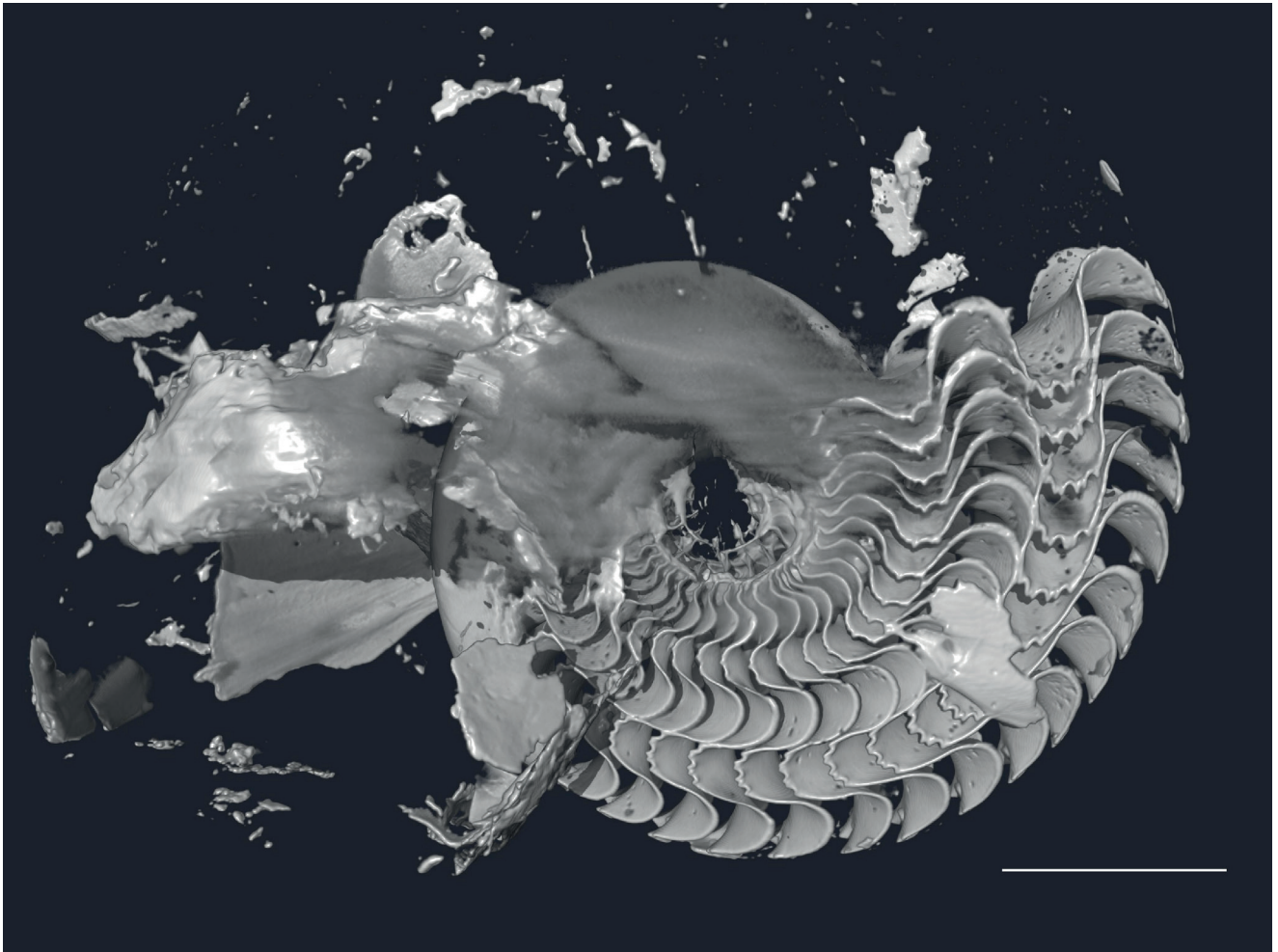
Figure 7. CT scan image of Prionitid sp., PMO 227.988, lateral view, body chamber on top. Outer shell not visible.
