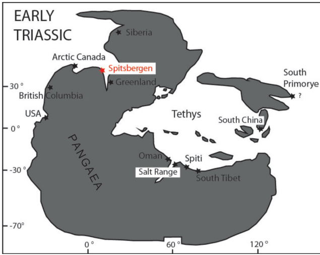
Figure 1. Early Triassic palaeogeographic setting. Spitsbergen (red star) as well as other important localities (black stars) is shown (modified from Brühwiler et al., 2010, fig. 1).
