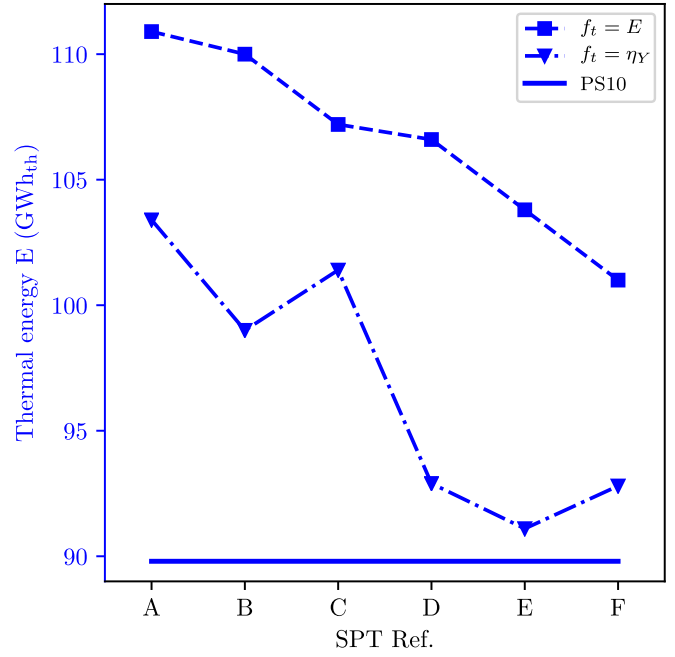
Fig. 4. Yearly thermal energy collected for each case.
