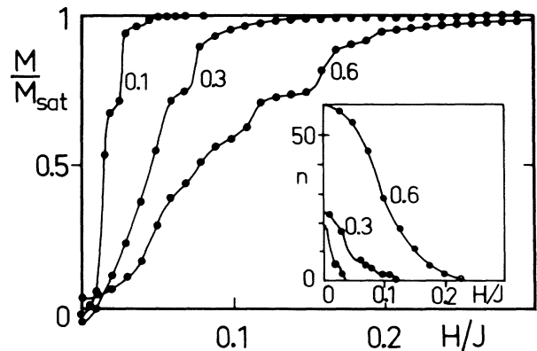
FIG. 5. First magnetization curves for three values of D/J : 0.1, 0.3, and 0.6. Inset: Number of vortices n vs the applied field H/J for the same values of D/J .
