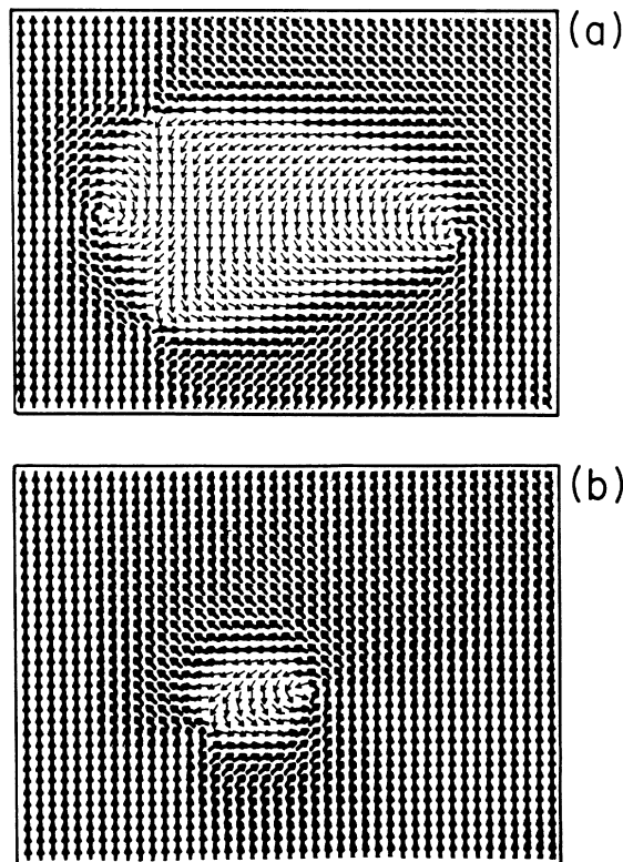
FIG. 6. Magnification of a part of the sample for D/J=0.1 and two consecutive values of the applied field: H/J=0.025 and 0.026 . Between these two stages of the magnetization process, a pair of vortices annihilated and another one shrunk.
