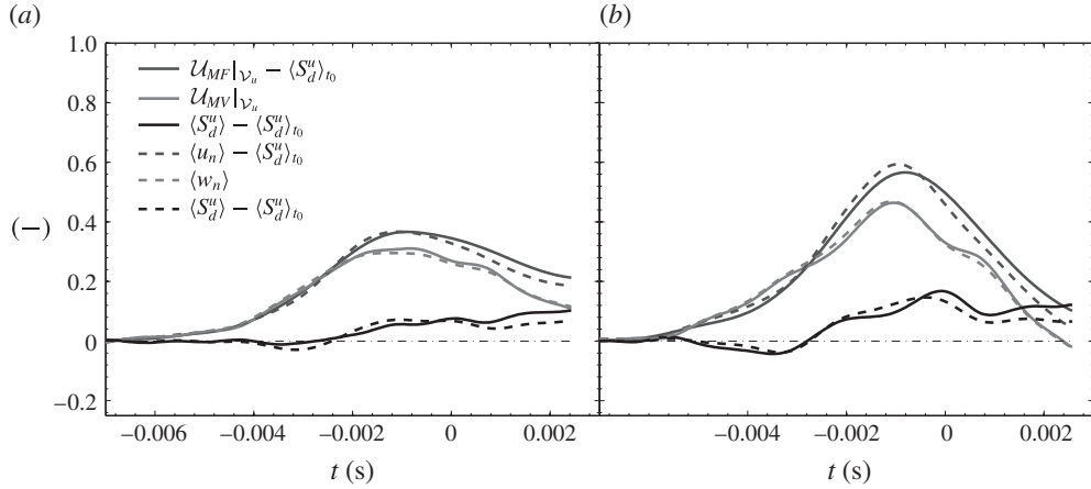
FIGURE 13. Validation of the estimation of the flame displacement speed for \Delta = 13 mm. Full line represent the different terms in (3.11) while the dashed line represents the area-weighted average of terms in (5.6a). All terms have been normalized by \langle S_d^u \rangle_{t_0} . (a) Methane/air U_\theta / \langle S_c^1 \rangle = 0.8 . (b) Propane/air U_\theta / \langle S_c^1 \rangle = 1.2 .
