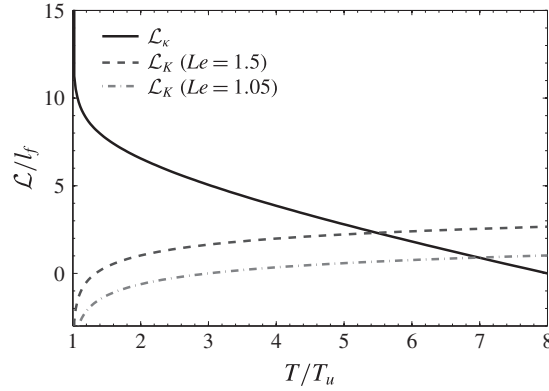
FIGURE 10. Evolution of the curvature and stretch Markstein length as a function of the reduced temperature as inferred from (1.8) with \beta = 8 , Le = 1.5/1.05 and \lambda = (T/T_u)^{0.87} .
