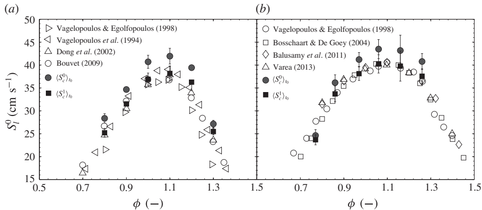
FIGURE 3. Comparison of the present experimental assessment of the consumption speed using (4.1) with \mathcal{F} = 0 (filled circle) and \mathcal{F} = \delta_L/2 (filled square), for methane (a) and propane/air mixtures (b) at different equivalence ratios \phi with data from the literature. Error bars correspond to the standard deviation calculated from 15 independent measurements. Experimental data are taken from Vagelopoulos et al. (1994), Vagelopoulos & Egolfopoulos (1998), Dong et al. (2002), Bosschaart & De Goeij (2004), Bouvet (2009), Balusamy et al. (2011) and Varea (2013).
