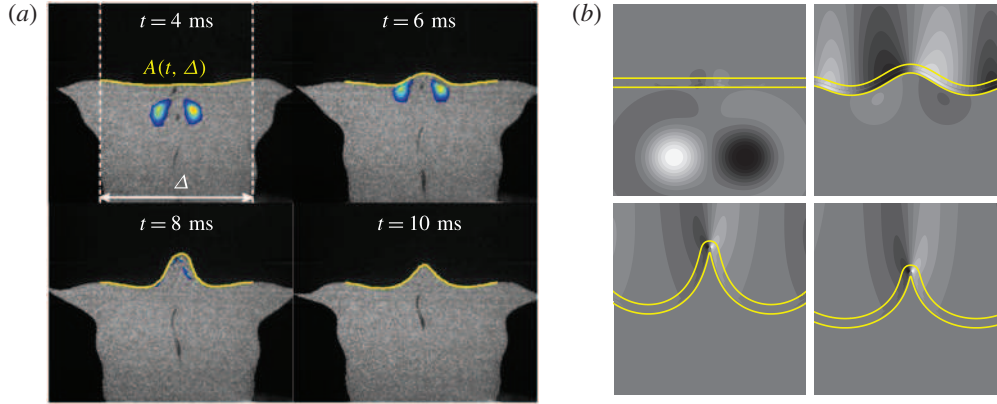
FIGURE 4. (Colour online) Time sequence of FVI. (a) Experimental contour of vorticity superimposed on the raw Mie scattering image together with one particular isotherm located close to the leading edge. (b) DNS contours of vorticity and the Y_f^* = 0.01 and Y_f^* = 0.99 iso-levels. For clarity, the DNS field has been symmetrically doubled and only a portion of the calculation domain is displayed in (b).
