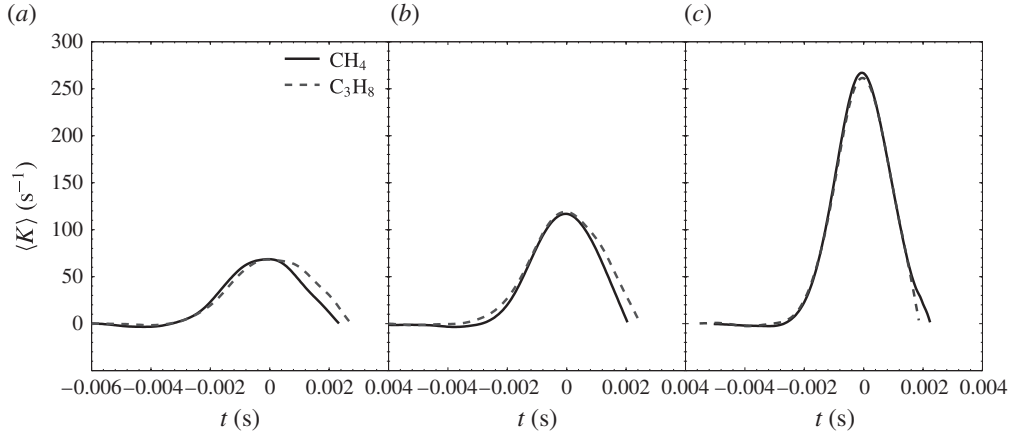
FIGURE 6. Time evolution of the stretch rate for stoichiometric methane and lean ( \phi = 0.9 ) propane/air mixtures for three different vortex strengths and \Delta = 13 mm: (a) U_\theta / \langle S_c^1 \rangle_{t_0} = 0.8 , (b) U_\theta / \langle S_c^1 \rangle_{t_0} = 1.2 , (c) U_\theta / \langle S_c^1 \rangle_{t_0} = 2.8 . The time t has been shifted so that t = 0 corresponds to the time at which \langle K \rangle is maximum.
