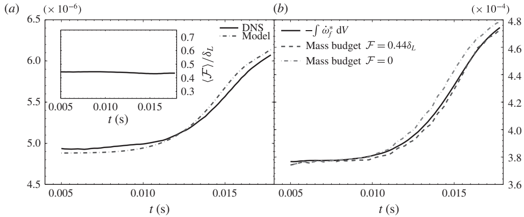
FIGURE 5. (a) Time evolution of the mass contained within the flame as inferred from the DNS (left-hand side of (4.4)) or the model with \mathcal{F} = \text{const.} = 0.44\delta_L (right-hand side of (4.4)). The figure in the inset represents the ratio \mathcal{F}/\delta_L . (b) Volume integrated fuel reaction rate as inferred from the DNS, compared with the mass budget using either \mathcal{F} = 0 or \mathcal{F} = \text{const.} = 0.44\delta_L . Using \mathcal{F} = \text{const.} = 0.5\delta_L was undistinguishable from \mathcal{F} = \text{const.} = 0.44\delta_L .
