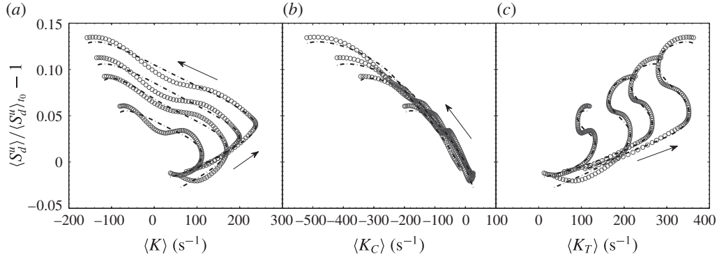
FIGURE 9. Plots of \langle S_d^u \rangle versus \langle K \rangle (a), \langle K_C \rangle (b) and \langle K_T \rangle (c) for methane/air mixture at U_\theta / \langle S_c^1 \rangle_{t_0} = 2.8 . The arrow indicates the direction of increasing time. The different curves correspond to different width \Delta of the control volume; the smaller \Delta the larger the variations of \langle S_d^u \rangle , \langle K \rangle , \langle K_C \rangle and \langle K_T \rangle . The dotted lines corresponds to predictions using (5.9) with \mathcal{L}_\kappa = 4.98l_f and \mathcal{L}_\kappa = -1.08l_f .
