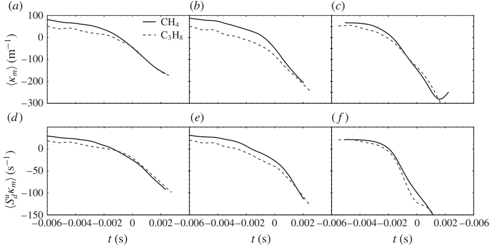
FIGURE 7. Time evolution of \langle \kappa_m \rangle (a–c) and \langle S_d^u \kappa_m \rangle (d–f) for stoichiometric methane and lean ( \phi = 0.9 ) propane/air mixtures for three different vortex strengths: (a,d) U_\theta / \langle S_c^1 \rangle_{t_0} = 0.8 , (b,e) U_\theta / \langle S_c^1 \rangle_{t_0} = 1.2 , (c,f) U_\theta / \langle S_c^1 \rangle_{t_0} = 2.8 . The time t has been shifted so that t = 0 corresponds to the time at which \langle K \rangle is maximum.
