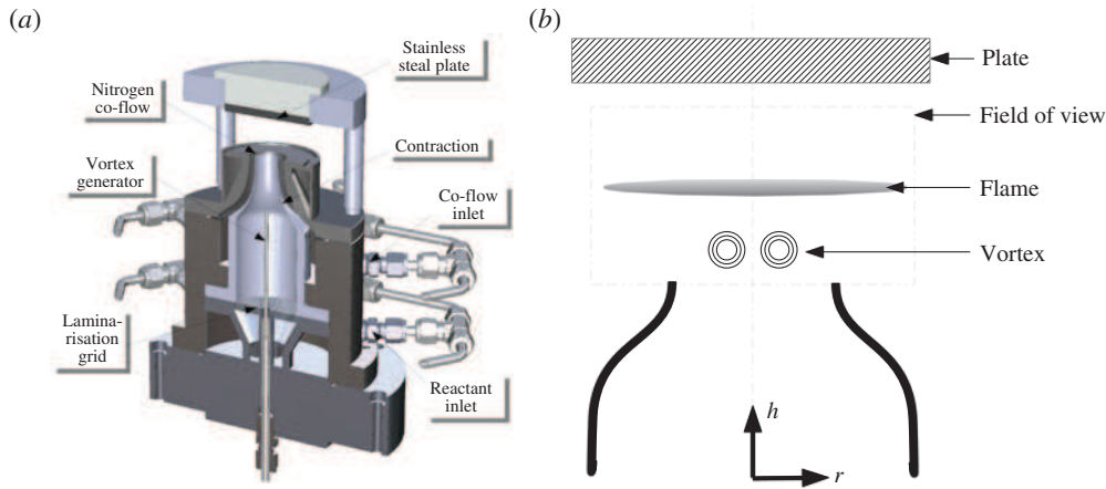
FIGURE 1. (Colour online) Schematic of the flame–vortex interaction burner (FVIB).
