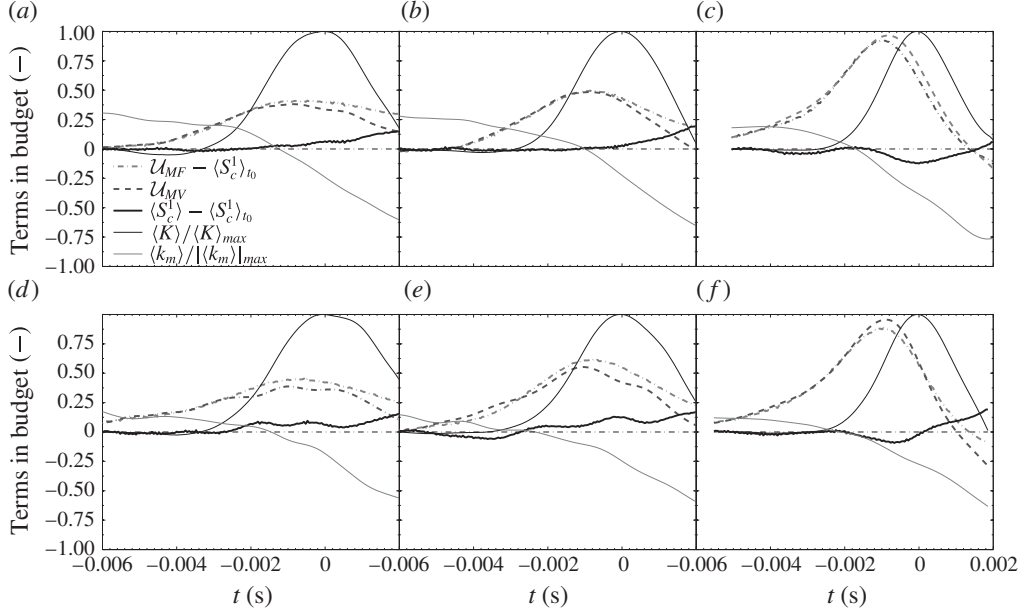
FIGURE 11. Time evolution of the different terms in (3.22) normalized by \langle S_c^1 \rangle_{t_0} . The vortex intensity U_\theta / \langle S_c^1 \rangle_{t_0} = 0.8 (a,d), 1.2 (b,e) and 2.8 (c,f). Stoichiometric \text{CH}_4/\text{Air} mixture (a–c), lean ( \phi = 0.9 ) \text{C}_3\text{H}_8/\text{Air} mixture (d–f).
