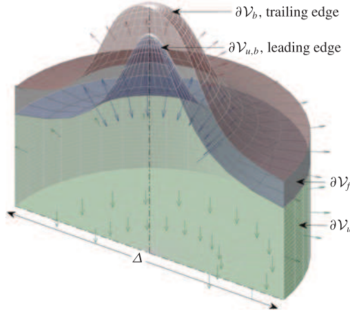
FIGURE 2. (Colour online) Schematic of (half) the material volume of diameter \Delta , over which (3.1) is integrated. The volume \mathcal{V} is divided into two parts, i.e. \mathcal{V} = \mathcal{V}_u + \mathcal{V}_b with boundaries \partial\mathcal{V} = \partial\mathcal{V}_u + \partial\mathcal{V}_b + \partial\mathcal{V}_f . The two volumes share a common frontier \partial\mathcal{V}_{u,b} . The vectors \mathbf{n} normal to the different boundaries are indicated by arrows.
