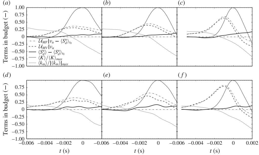
FIGURE 8. Time evolution of the different terms in (3.11), normalized by \langle S_d^u \rangle_{t_0} . The vortex intensity U_\theta / \langle S_c^1 \rangle_{t_0} = 0.8 (a,d), 1.2 (b,e) and 2.8 (c,e). Stoichiometric \text{CH}_4/\text{Air} mixture (a–c), lean ( \phi = 0.9 ) \text{C}_3\text{H}_8/\text{Air} mixture (d–f). The time t is translated so that t = 0 corresponds to the maximum of total stretch rate.
