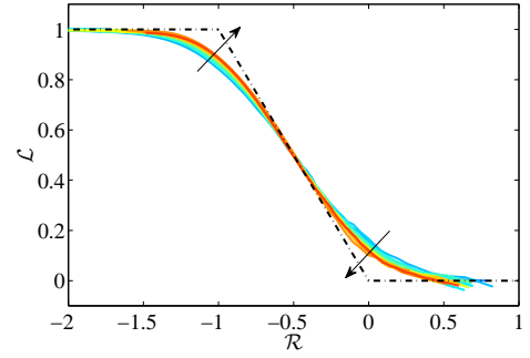
FIG. 10. (Color online). (a) Scale entropy \mathcal{L}(\mathcal{R}) as defined by Eq. (15). The black dash-dotted lines represents the asymptotic distribution, i.e. a \rightarrow \infty .
