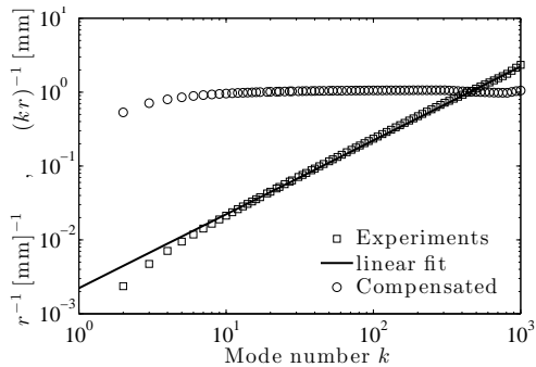
FIG. 5. Correspondance between mode numbers k and wavenumbers r^{-1} for Flame 18 (Table I). A clear linear slope, i.e. r^{-1} \propto k is observed as also confirmed by the compensated wavenumber (kr)^{-1}
