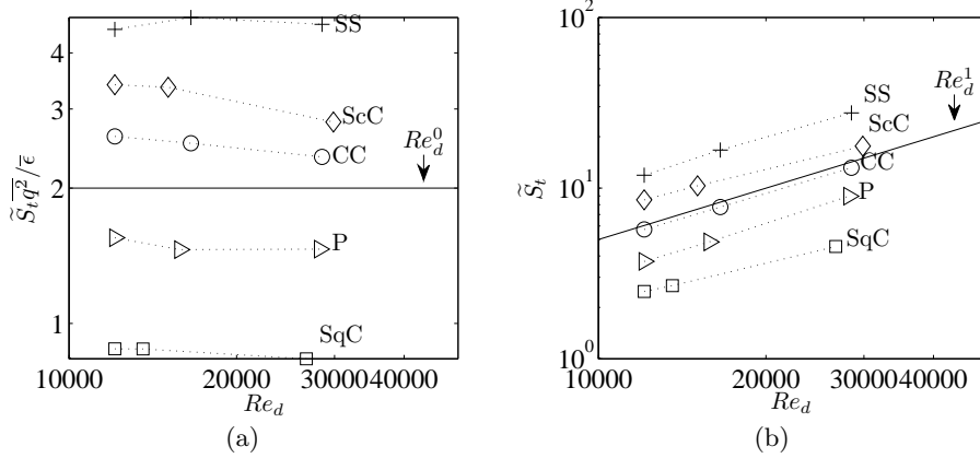
FIGURE 8. (a) \tilde{S}_t \overline{q^2} / \bar{\epsilon} , — : Re_d^0 . (b) Absolute value of the coherent shear \tilde{S}_t for various Reynolds numbers, — : Re_d^1 , ○ CC, □ SqC, ◇ ScC, ▷ P, + SS.
