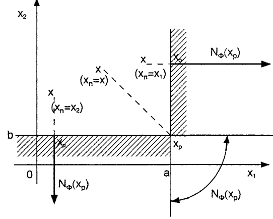
Fig. 4. Controllability in the normal cone.
