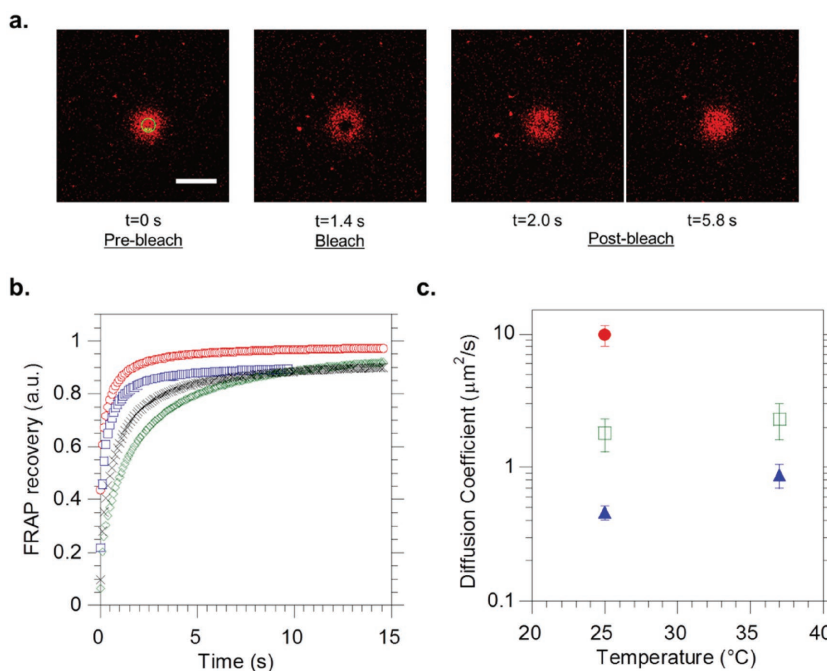
Figure 5. FRAP measurements on DOPE-rhodamine inserted into the membrane of PBut 2.5 - b -PEO 1.3 and asymmetric POPC/PBut 2.5 - b -PEO 1.3 (aGHUV) giant vesicles. a) Confocal images of a vesicle during the three phases of FRAP experiment, namely prebleach, bleach, and postbleach. We observe the recovery of fluorescence inside the ROI with time. Scale bar: 10 μm. b) Normalized fluorescence intensity profiles during recovery. Pure PBut 2.5 - b -PEO 1.3 giant vesicles (25 °C green, 37 °C black), POPC/PBut 2.5 - b -PEO 1.3 aGHUV (25 °C red, 37 °C blue). c) Measured lipid lateral diffusion coefficients ( D (μm 2 s -1 )) for different membranes and temperatures: pure POPC giant vesicles (●) (ref. [39]), POPC/PBut 2.5 - b -PEO 1.3 aGHUV (□), pure PBut 2.5 - b -PEO 1.3 giant vesicles (▲). Measurements were performed and averaged on 5–10 vesicles for each system.
