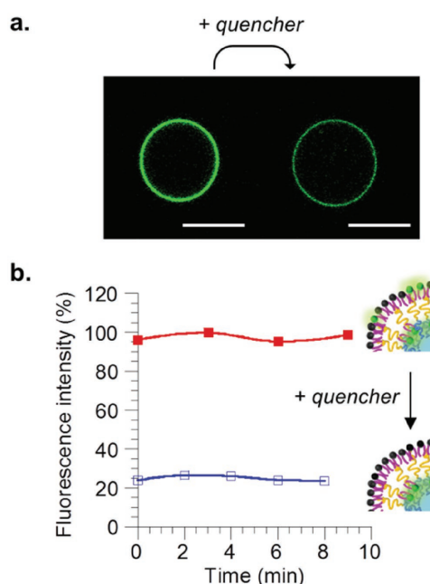
Figure 3. Spectral and microscopy analysis of POPC/ PBUT 2.5 -b-PEO 1.3 asymmetric vesicle solution incorporating PE-NBD on both sides of the membrane, before and after addition of dithionite as fluorescence quencher. a) Confocal microscopy observations before (left column) and after (right column) addition of dithionite. Scale bar = 10 μm. b) Fluorescence intensity of vesicle solution before (■) and after (□) addition of quencher.
