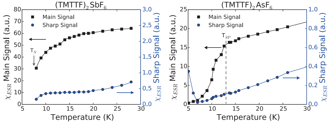
Figure 2: Intensity of CW EPR signals of (TMTTF) 2 SbF 6 (left) and (TMTTF) 2 AsF 6 (right). The Black squares and blue circles are intensities the main line and sharp line respectively.
