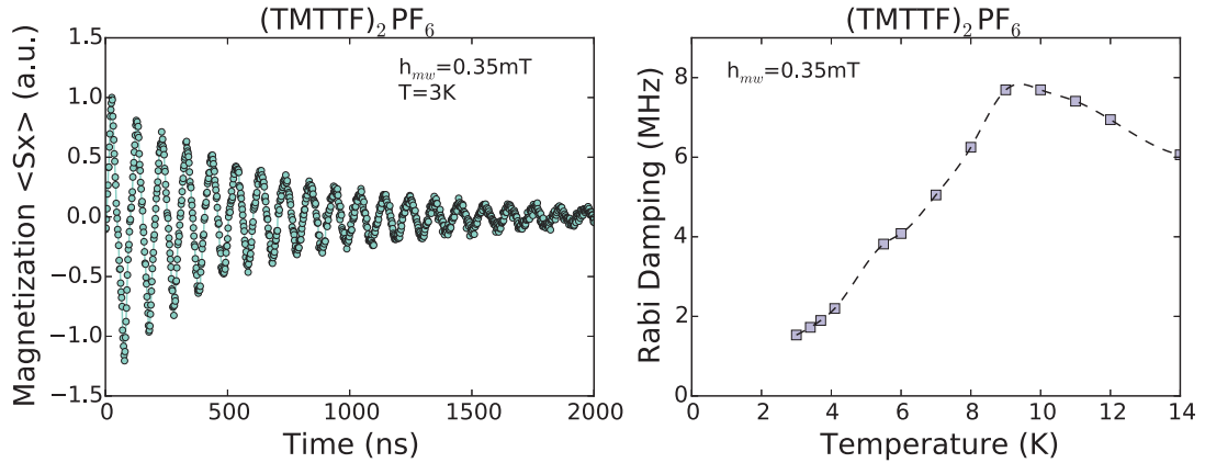
Figure 3: (left) Rabi oscillation of the strongly correlated defect observed in (TMTTF) 2 PF 6 at T=3 K. (right) Rabi damping obtained from the fits of Rabi oscillations of the pinned solitons for temperature below 14 K. Dashed line is a guide for the eyes.
