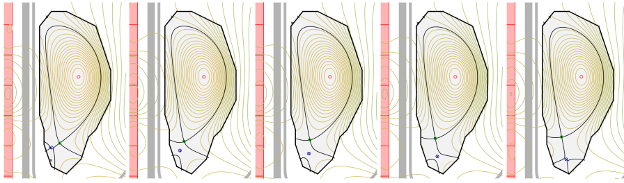
Fig. 13 The solutions of the optimal control problem with objective functional K(w; \psi) = K_1(\psi) + 1000K_2(\psi) and \mathbf{x}_0 is indicated by the blue circle.
