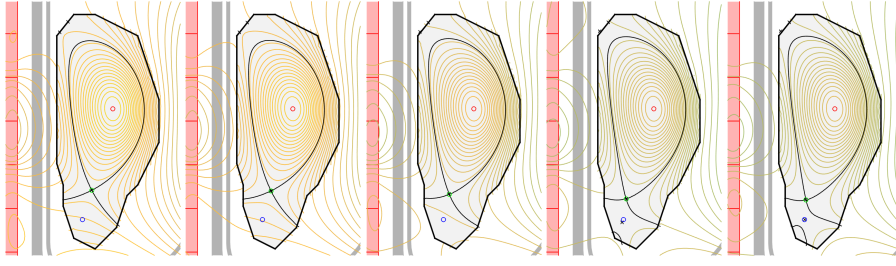
Fig. 11 The solutions of the optimal control problem with objective functional K(w; \psi) = K_1(\psi) + wK_2(\psi) and w = 0, 1, 10, 100, 1000 (from left to right), \mathbf{x}_0 is indicated by the blue circle.
