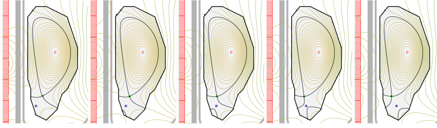
Fig. 12 The solutions of the optimal control problem with objective functional K(w; \psi) = K_1(\psi) + 1000K_2(\psi) and \mathbf{x}_0 is indicated by the blue circle.
