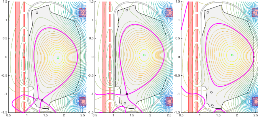
Fig. 9 Contour lines of the magnetic flux \psi for three different configuration of HL-2M. The location (r_{\max}(\psi), z_{\max}(\psi)) of the maximum of \psi is indicated with a green circle. The location (r_X, z_X) of the discrete saddle points of \psi is indicated by black circles. The magenta line indicates the contour line that contains the plasma boundary.
