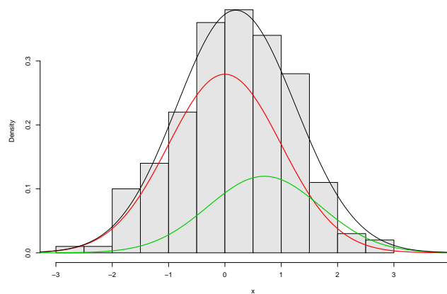
Figure 3: Typical empirical distribution of a n = 200 sample from the mixture model (5), with the true distributions for the two components (red, green) and the mixture (black).
