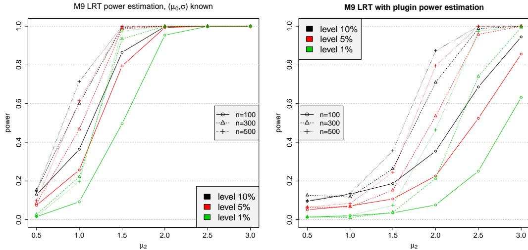
Figure 10: Monte-Carlo estimation of the power of the LRT for M9 , \lambda_n(\mathbf{x}, \mu_0, \sigma^2) , i.e. when (\mu_0, \sigma^2) are known (Left), and of \lambda_n(\mathbf{x}, \hat{\mu}_0(\mathbf{x}), \hat{\sigma}^2(\mathbf{x})) , i.e. LRT with plug-in (Right), as a function of the mean \mu_2 of the second component; a = 3 , 2000 replications.
