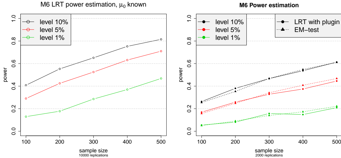
Figure 7: Monte-Carlo estimation of the power for M6 , H_1 as in Equation (5). Left : LRT using asymptotic definition of the statistic, i.e. \mu_0 known. Right : LRT with plug-in estimate based on the same sample, compared with the EM-test.
