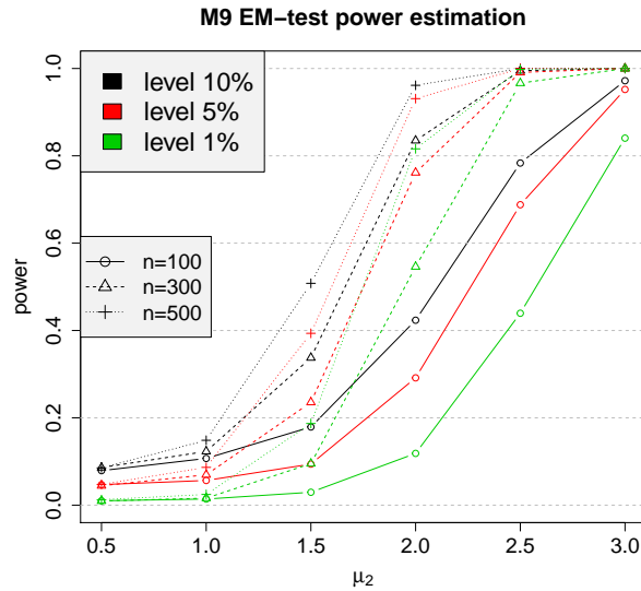
Figure 11: Monte-Carlo estimation of the power of the EM-test for M9 based on our implementation and 2000 replications, as a function of the mean \mu_2 of the second component.
