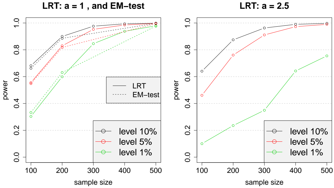
Figure 4: Power estimates for M2 . LRT: using the quantiles obtained by Monte-Carlo as in Figure 2, for a = 1 (left) and a = 2.5 (right), 10, 000 replications. EM-test (left): for n = 100, 200 and 500 , 2000 replications.
