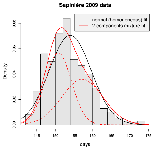
Figure 12: Homogeneous and 2-components mixture fits for the data Romane Sapinière 2009 .
