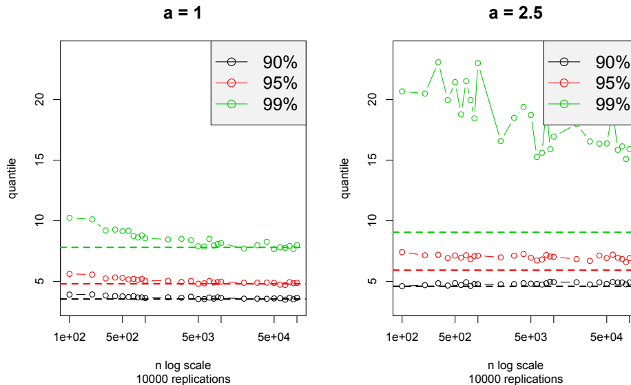
Figure 2: M2 : Empirical quantiles for \lambda_n based on 10,000 Monte-Carlo replications vs. Asymptotic theoretical values from Garel (2013) (dotted lines) for three percentiles (90%, 95% et 99%) and two compact sets with a = 1 (left) and a = 2.5 (right). The x axis is in log scale, for 100 \leq n \leq 100,000 .
