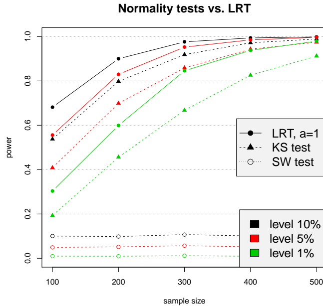
Figure 5: Power estimates for M2 : LRT vs. the KS and SW normality tests, 10,000 replications.
