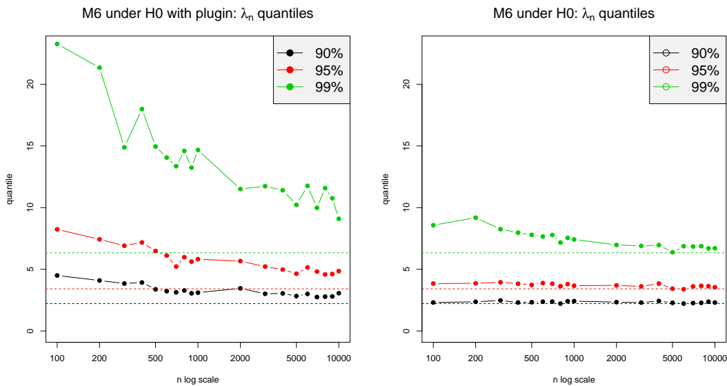
Figure 6: M6 Empirical quantiles of the LRT statistic for three percentiles (90%, 95% et 99%), a = 1 . Left: for \lambda_n(\mathbf{x}, \hat{\mu}_0(\mathbf{x})) , 2000 replications; Right: for \lambda_n(\mathbf{x}, \mu_0) , 10,000 replications. Dotted lines are asymptotic values from Garel (2013). The n axis is in log scale.
