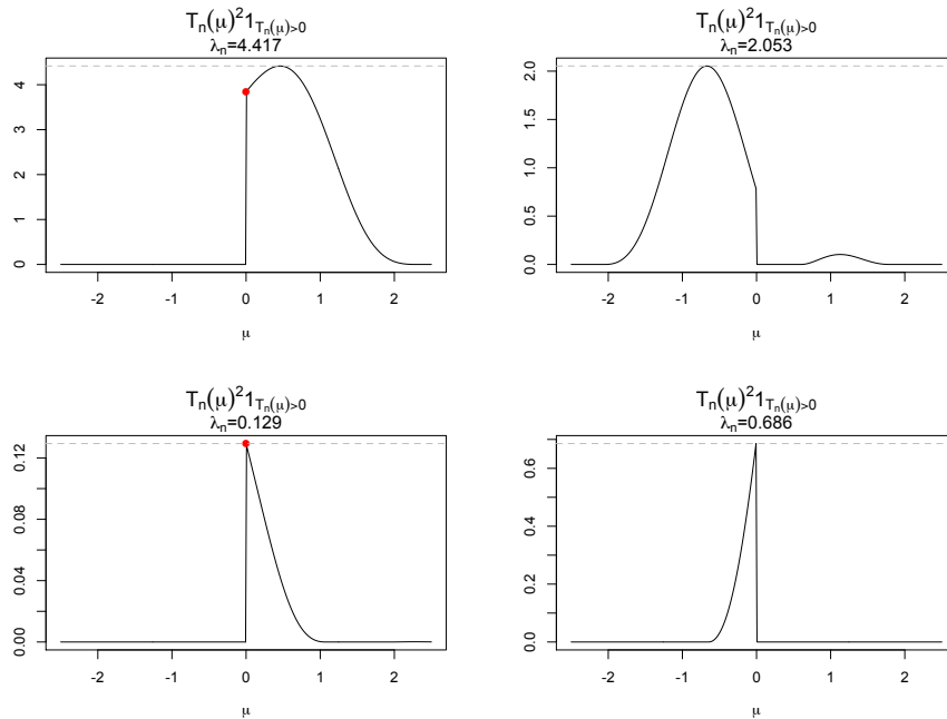
Figure 1: Some typical behaviours of \mu \mapsto T_n^2(\mu) \mathbb{1}_{\{T_n(\mu) \geq 0\}} for a = 2.5 and simulated samples of size n = 1000 under H_0 for M2 . The red dot is the limiting behaviour T_n^2(0) , when T_n(0) \geq 0 .
