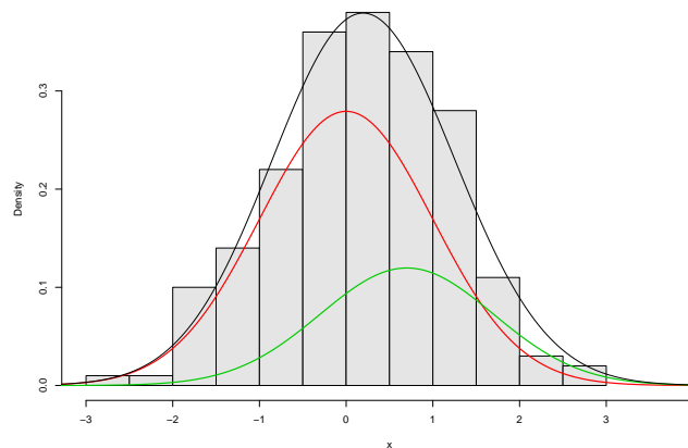
Figure 3: Typical empirical distribution of a n = 200 sample from the mixture model (4), with the true distributions for the two components (red, green) and the mixture (black).
