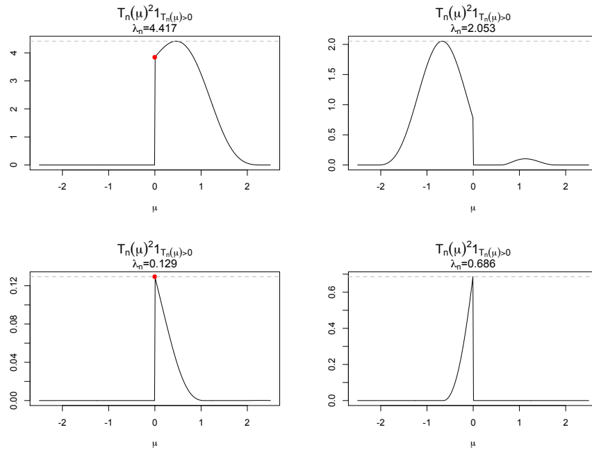
Figure 1: Some typical behaviours of \mu \mapsto T_n^2(\mu)\mathbb{I}_{\{T_n(\mu) \geq 0\}} for \mu \in [-2.5, +2.5] and simulated samples of size n = 1000 under H_0 for (M2). The red dot is the limiting behaviour T_n^2(0) , when T_n(0) \geq 0 .
