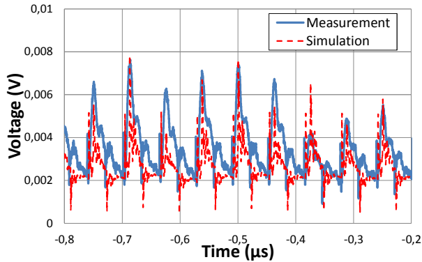
Fig. 16. Comparison between the measured and simulated external voltage using a 1 \Omega probe in the time domain using the statistical approach (5-bit PRNG configuration)
