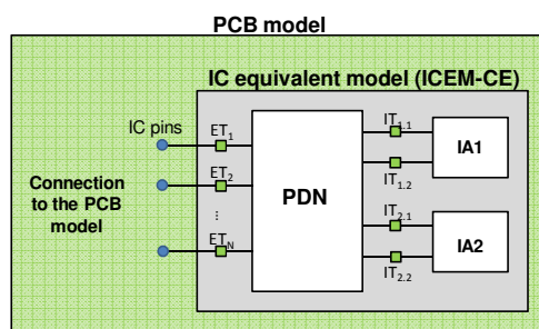
Fig. 1. Structure of ICEM-CE model
