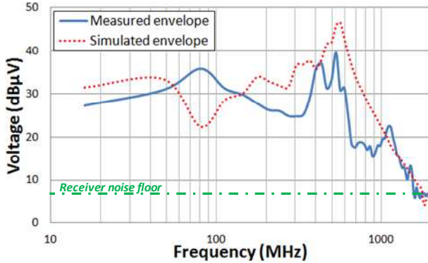
Fig. 20. Comparison between the measured and simulated spectral envelope CE with a 150 Ω probe on 1.2 V power plane (Industrial Application)
