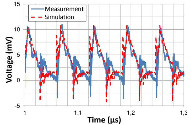
Fig. 18. Comparison between the measured and simulated external voltage with a 1 \Omega probe in the time domain (Industrial Application)
