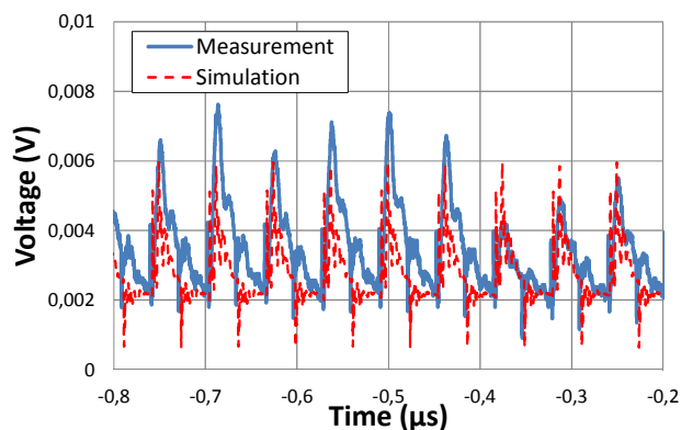
Fig. 14. Comparison between the measured and simulated external voltage using a 1 \Omega probe in the time domain using the deterministic approach (5-bit PRNG configuration)
