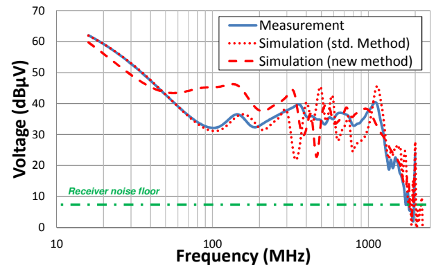
Fig. 22. Comparison between the measured and simulated spectral envelope CE with a 1 Ω probe according to the standard and new IA extraction method (Delay Line configuration)
