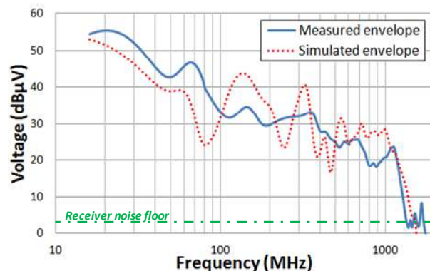
Fig. 15. Comparison between the measured and simulated external voltage using a 1 \Omega probe in the frequency domain using the deterministic approach (5-bit PRNG configuration)
