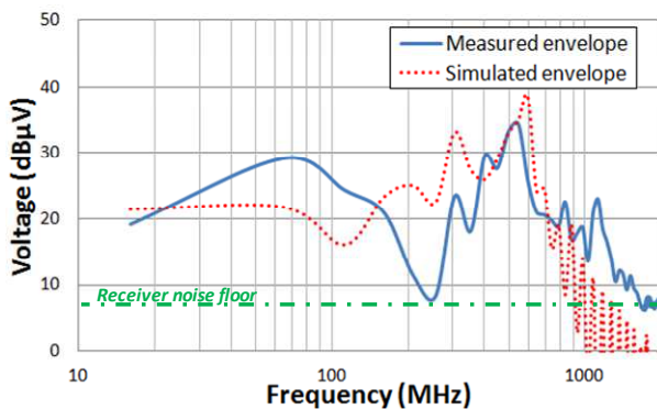
Fig. 17. Comparison between the measured and simulated spectral envelope CE with a 150 \Omega probe on 1.2 V power plane (5-bit PRNG configuration)
