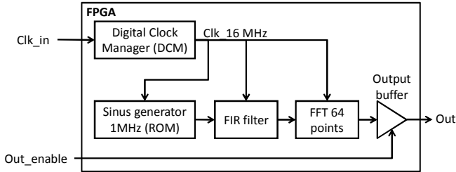
Fig. 9. Structure of the industrial application case study
