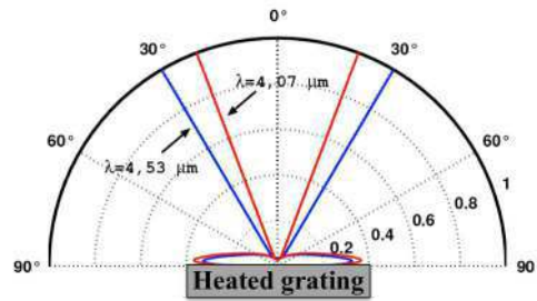
Figure 2. Emissivity of a tungsten lamellar grating. Period p = 3 \mu\text{m} , filling factor F = 0.5 and height of the lines h = 125 \text{ nm} . The emissivity angular diagram is calculated for two different indicated wavelengths and shows very directional peaks (from [18]).
