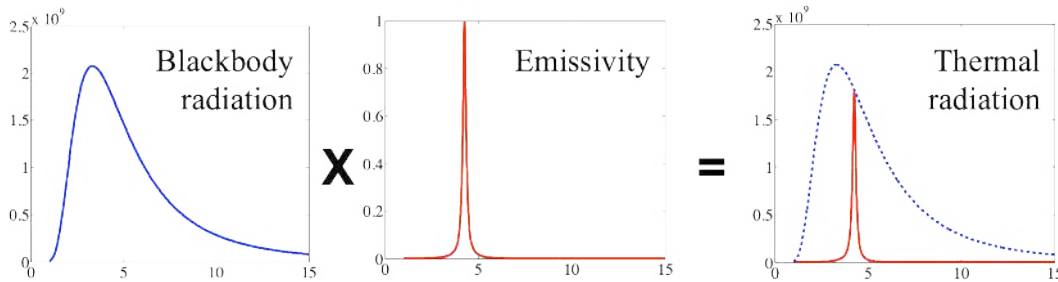
Figure 1. Illustration of the concept of emissivity in the wavelength domain. Compared to the case of a black-body at a given temperature (blue curve on the left, here given at a temperature of 600°C as a function of the wavelength in micrometers), the radiance from a real thermal source is given by the product of this blackbody radiance by the emissivity (Red curve in the middle), which is a function of the wavelength and (not shown) the direction of emission. When the emissivity equals unity, the radiance of the source is maximal.
