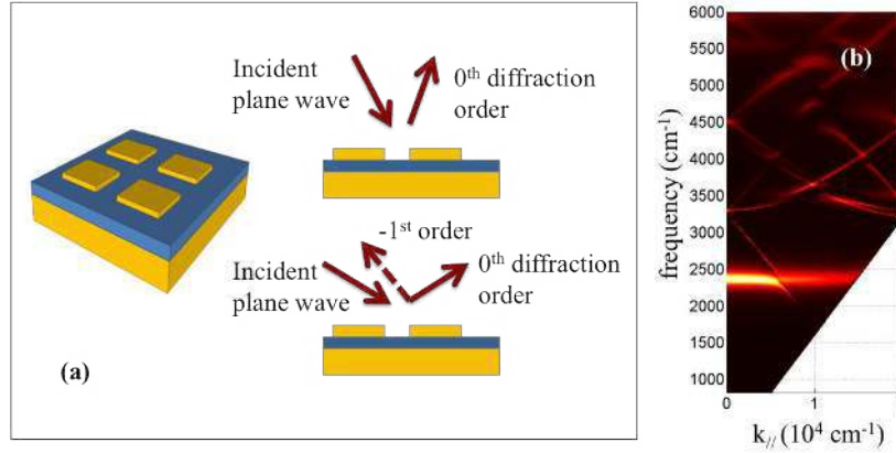
Figure 4. (a) Directional features are obtained taking advantage of diffraction orders appearance beyond cut-off angles. For small k_{//} values, a single specular order exists whereas for larger values other diffraction orders appear leading to additional radiative channels. The critical coupling (i.e. the attainment of a maximum close to 100% in Fig.3) is not fulfilled anymore, and the absorption decreases. (b) Calculated absorptivity as a function of the frequency and the incident k_{//} vector. The absorptivity is averaged over the two polarizations. The simulated structure is characterized by the gold-square side L = 900 nm, dielectric thickness h = 120 nm and period p = 3 \mu\text{m} of the array.
