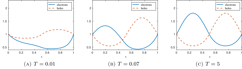
FIGURE 3. Evolution of approximate densities in Case 1, for C piecewise constant with \|C\|_\infty = 20 .
