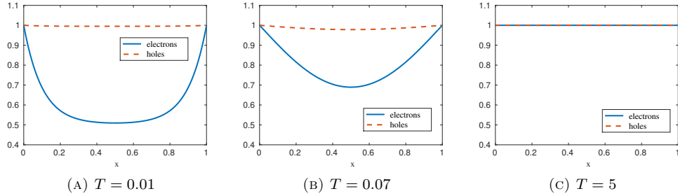
FIGURE 1. Evolution of approximate densities in Case 1, for C = 0 .
