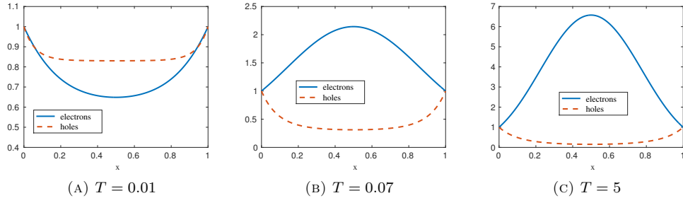
FIGURE 2. Evolution of approximate densities in Case 1, for C = 20 .
