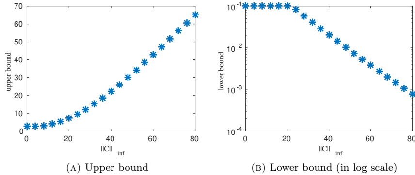
FIGURE 6. Upper and lower bounds as functions of \|C\|_\infty in Case 2, with C given by (61).
