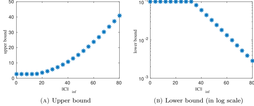
FIGURE 7. Upper and lower bounds as functions of \|C\|_\infty in Case 2, with C given by (62).
