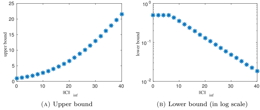
FIGURE 4. Upper and lower bounds as functions of \|C\|_\infty in Case 1, with C given by (59).
