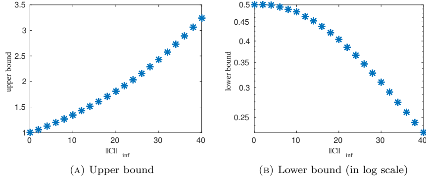
FIGURE 5. Upper and lower bounds as functions of \|C\|_\infty in Case 1, with C given by (60).
