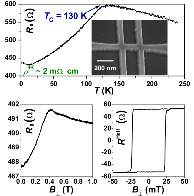
FIG. 1 (color online). (Top) Temperature dependence of the square resistance measured with a GaMnAs nano-Hall bar ( L = 220 \text{ nm} , W = 50 \text{ nm} ), a common behavior for both anisotropy. (Bottom left) Anisotropic magnetoresistance at T_{\text{cryo}} = 25 \text{ mK} , for an in-plane anisotropy. (Bottom right) Extraordinary Hall resistance at T_{\text{cryo}} = 25 \text{ mK} , for a perpendicular anisotropy. All measurements were done with a large current I = 100 \text{ nA} , leading to vanishingly small quantum corrections (see text).
