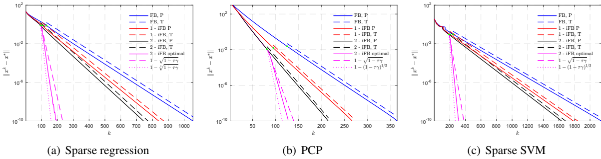
Figure 1: Finite identification and local linear convergence of MiFB under different inertial settings in terms of \|x_k - x^*\| . “P” stands for practical observation and “T” indicates the theoretical estimate. We fix \gamma_k \equiv 0.3/L for all tests. For the 2 inertial schemes, inertial parameters are first chosen such that (2.3) holds. The position of the green dot in each plot indicates the iteration beyond which identification of \mathcal{M}_{x^*} occurs.
