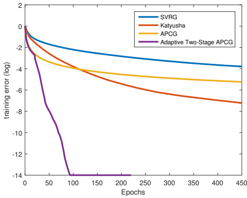
(c) \lambda = 2 \times 10^{-3} , \|x^*\|_0 = 636
