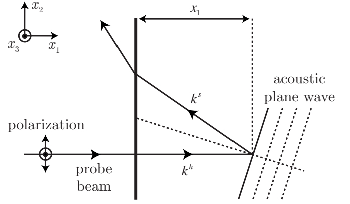
FIG. 1. Interaction of the normal incidence probe beam with a single plane wave propagating in an oblique direction.
