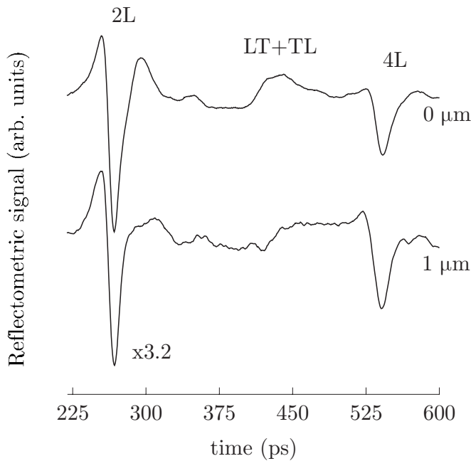
FIG. 2. Measured reflectometric signal in an isotropic aluminum film deposited on Mylar for pump-probe distances of 0 and 1 \mu\text{m} . Longitudinal waves 2L and 4L, together with the mode converted TL and LT waves, are observed.
