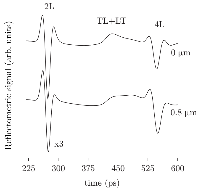
FIG. 3. Calculated reflectometric signal in a free isotropic aluminum film for different pump-probe distances: 0 and 0.8 \mu\text{m} . Longitudinal waves 2L and 4L, together with the mode converted TL and LT waves, can be observed.
