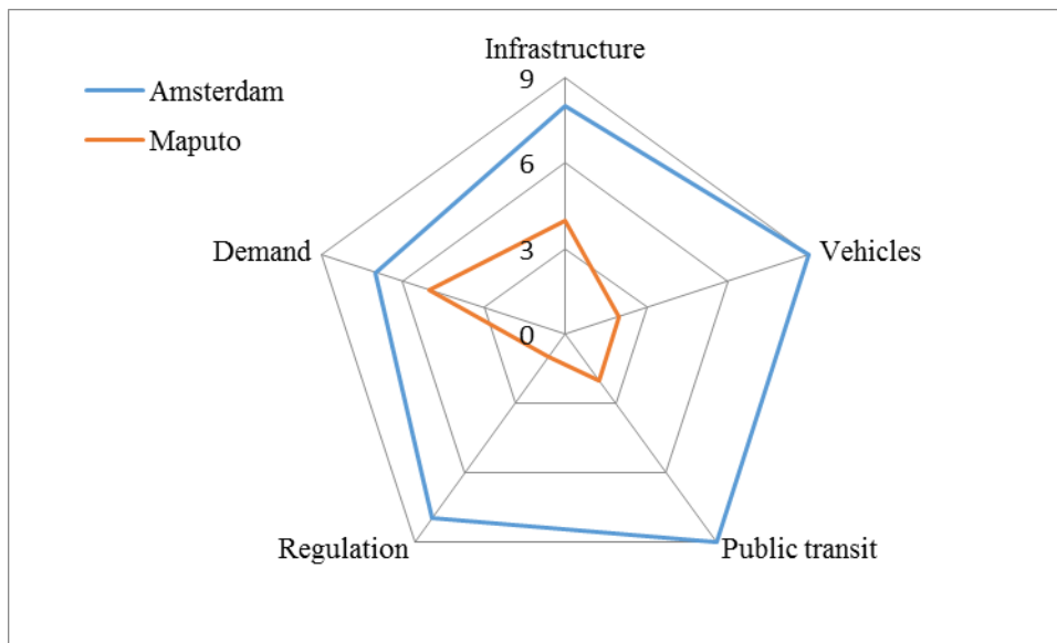
1 2 3 FIGURE 3 Radar chart – two city samples
