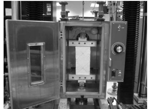
Fig. 31. A bias-extension sample in an oven.
