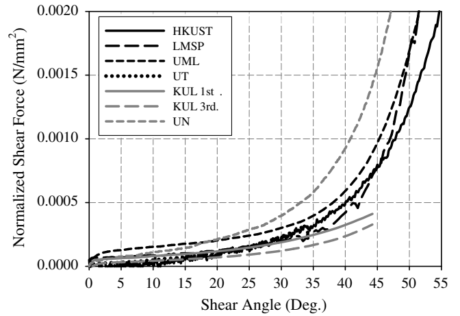
Fig. 27. Shear force normalized by the inner fabric area vs. shear angle.
