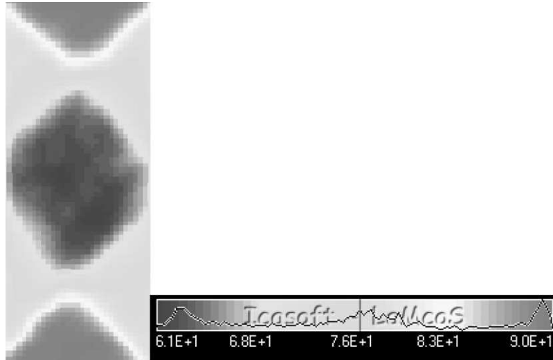
Fig. 37. Contour of shear angle in a plain weave fabric with a sample size in a bias-extension test obtained from the optical measurement software Icasoft (INSA-Lyon/NU).
