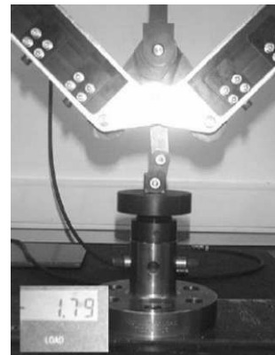
Fig. 18. Hinge for calibrating the force required to deform the frame.
