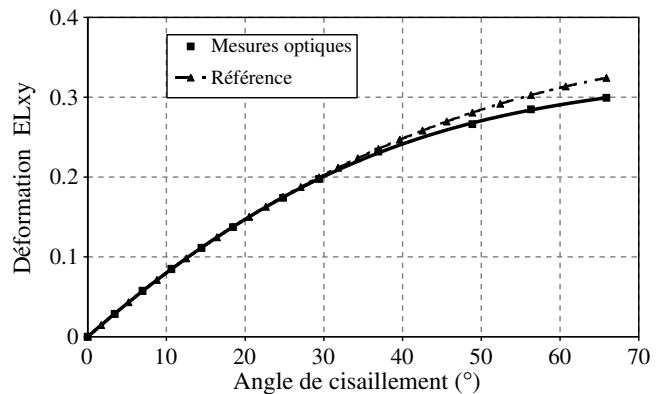
Fig. 17. A comparison between global strain component \epsilon_{xy} measured with optical device and the theoretical strain corresponding to frame kinematics (LMSP).
