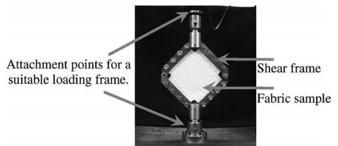
Fig. 4. Trellising-shear test apparatus.
