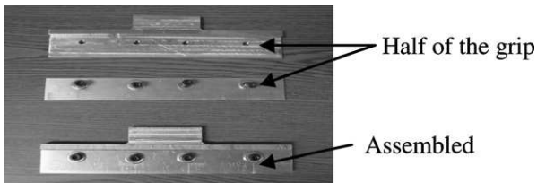
Fig. 33. A picture of the grips used at NU's bias-extension tests.
