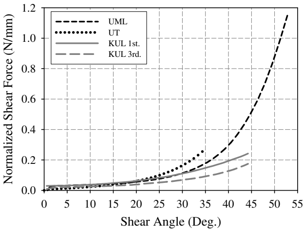
Fig. 29. Normalized shear force vs. global shear angle of the balanced twill-weave fabric.
