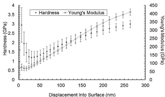
Figure 8. Average values of the mechanical properties of the Ti/Cr/Au metallization scheme as obtained using DCM indenter.
