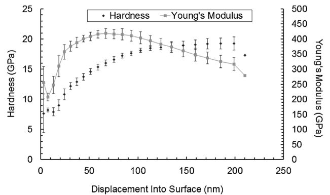
Figure 9. Average values of the mechanical properties of the Ti/Cr metallization scheme as obtained using DCM indenter.
