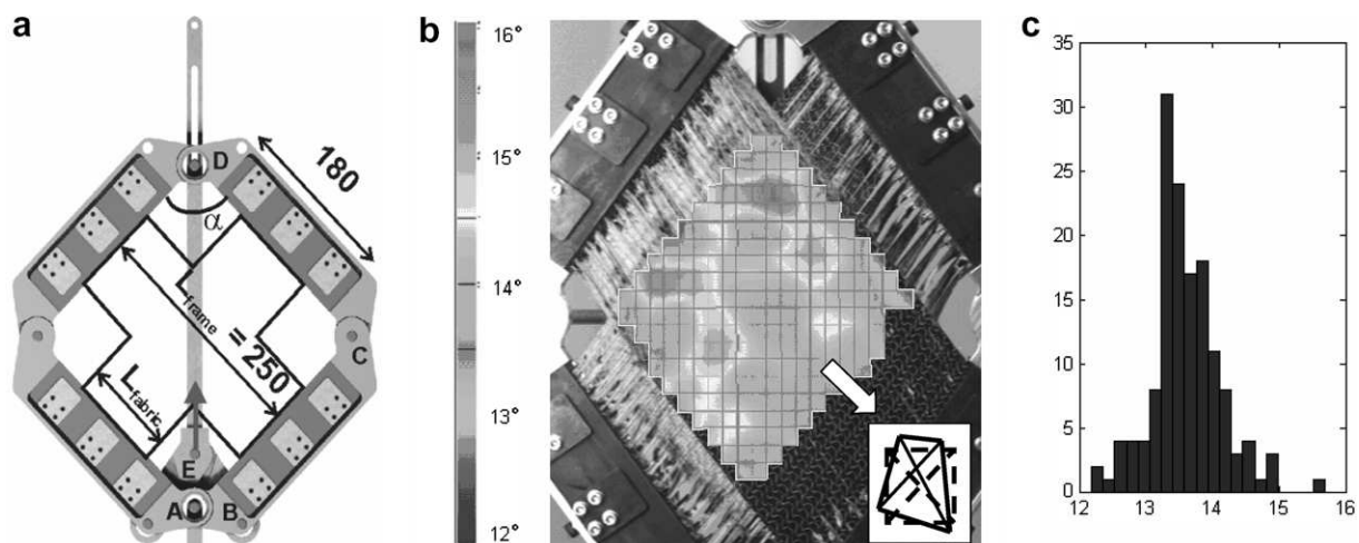
Fig. 1. Picture frame: (a) the device; (b) typical shear angle field for fabric B2, frame shear angle 14^\circ ; inset: scheme for calculation of the local shear angle (c) histogram of the distribution of the shear angle (frame shear angle 14^\circ ).
