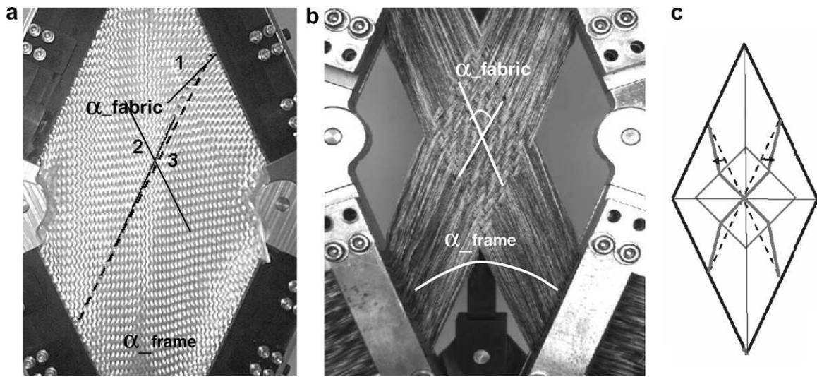
Fig. 2. Two types of samples on picture frame: (a) large sample, fabric shear is higher then the frame shear; (b) small sample, yarns in the “arms” are drawn out, fabric shear is less then the frame shear; (c) scheme of the positions of the yarns in the case (b).
