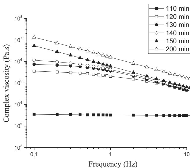
Fig. 5. Dynamic (complex) viscosity versus frequency at different crosslinking times for the HTA.
