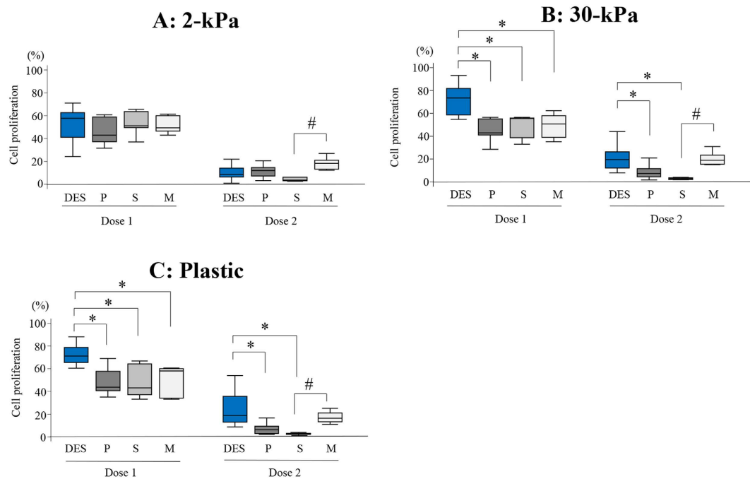
Figure 5. Comparison of cell proliferation of DES (n = 14), EES-P (n = 10), EES-S (n = 6) and EES-M (n = 5) grown on PGS of varying stiffness (2 (A) or 30 kPa (B)) or plastic (C) after a 72-h discontinuation of U0126 and MK2206. P: EES-P. S: EES-S. M: EES-M. Dose 1: U0126 (15 \mu M) and MK2206 (4.5 \mu M). Dose 2: U0126 (30 \mu M) and MK2206 (9 \mu M). *p < 0.05 versus DES. #p < 0.05 versus EES-M. Numerical values are presented as box and whisker plots showing medians and the smallest and largest data points \leq 1.5 \times IQR from the 25th and 75th percentiles, respectively.
