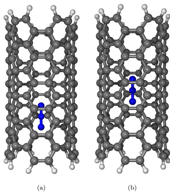
Fig. 4 Starting (a) and final (b) position of the N_3^- ion inside the CNT
