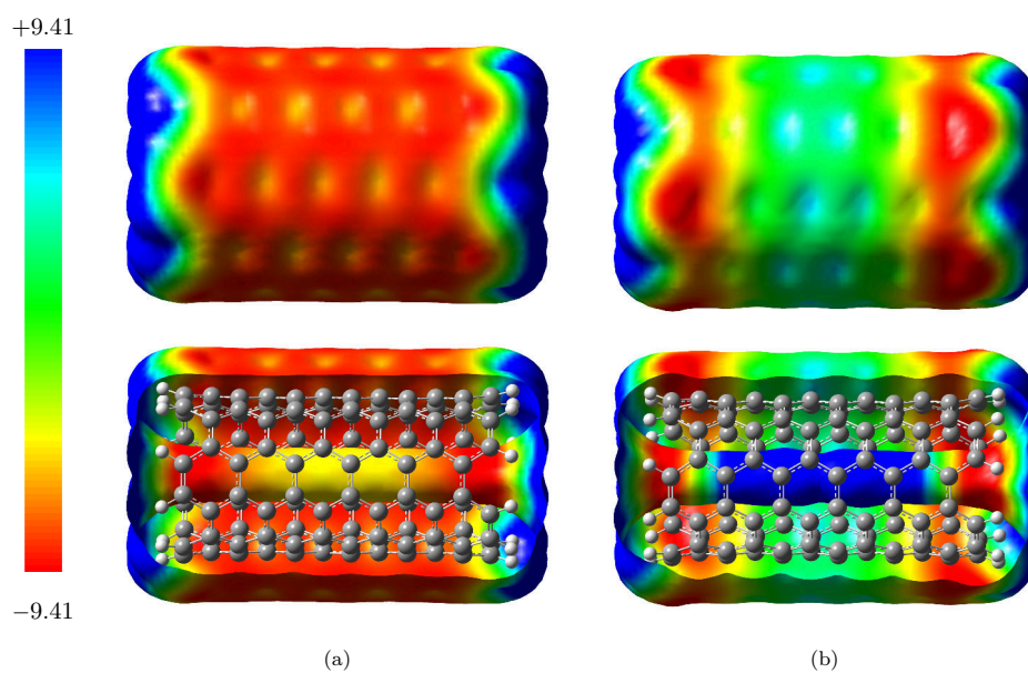
Fig. 8 Electrostatic potential map of the (5,5) CNT unperturbed (a) and perturbed by the presence of the N 3 - molecule (b). Isosurface value of the electron density set to 0.02 and energy scale given in kcal/mol
