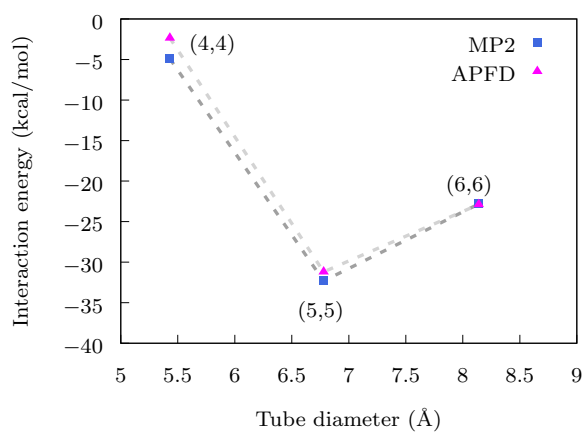
Fig. 6 Relaxed interaction energies
