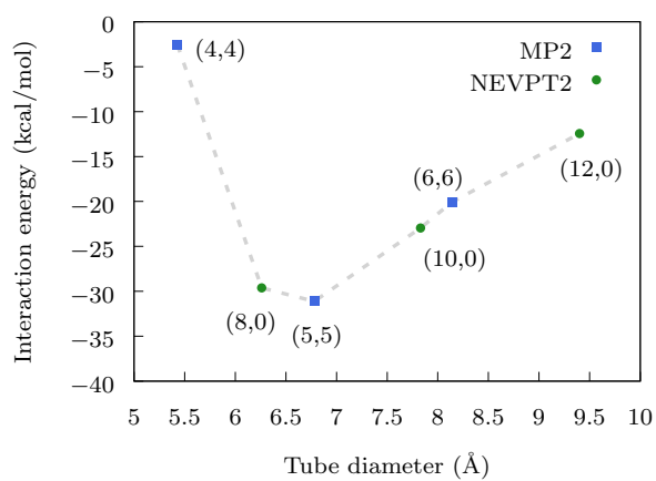
Fig. 2 Unrelaxed interaction energies
