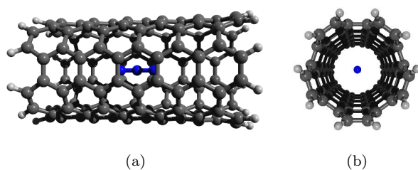
Fig. 1 Example geometry of N 3 - confined inside a (5,5) CNT used to compute unrelaxed interaction energies
