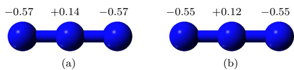
Fig. 7 Partial atomic charges for the N_3^- fragment outside (a) and inside a (5,5) CNT (b)
