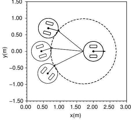
Fig. 5: Multiple positions of the follower robot for the same tether slackness and orientation: the problem only constrains the tether shape and orientation w.r.t. the follower robot
