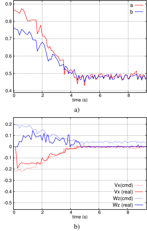
Fig. 7: Results of a real experiment for tether shape control. (a) the tether parameters evolution. The tether goes from an initial to a desired shape ( \mathbf{s}_o = (0.9, 0.8) and \mathbf{s}^* = (0.5, 0.5) , respectively). (b) the control velocities. Linear velocity ( v_x ) in m/s and angular velocity ( w_z ) in rad/s
