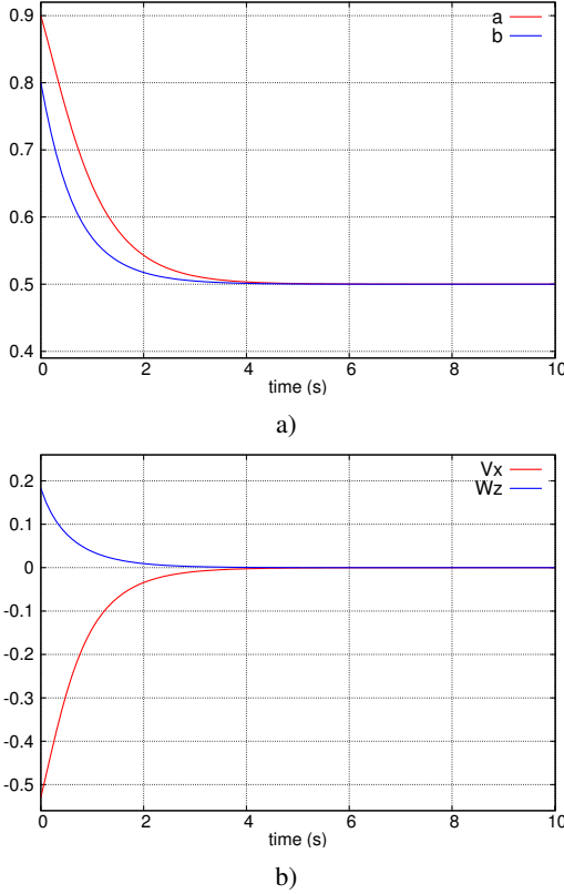
Fig. 6: Simulation results for tether shape control. (a) the parameters evolution. The tether goes from an initial to a desired shape ( \mathbf{s}_o = (0.9, 0.8) and \mathbf{s}^* = (0.5, 0.5) , respectively). (b) the control velocities. Linear velocity ( v_x ) in m/s and angular velocity ( w_z ) in rad/s
