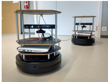
Fig. 1: Experimental setup: two Turtlebots [19] simulate a tether handling system for remotely operated robots. The leader robot freely explores its surroundings while the follower robot is expected to maintain the tether slack enough not to hamper the leader movements
