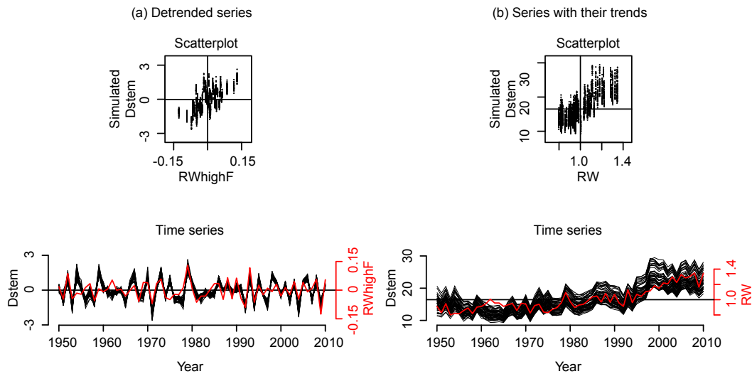
Figure 5. Comparison between the observed mean series of black spruce ring growth (unitless growth indexes) and MAIDEN-simulated carbon allocation to the stem (Dstem; \text{g C m}^{-2} \text{ yr}^{-1} ). (a) Detrended series (in the scatterplot the R^2 computed on data transformed to z scores is 0.24; r = 0.62 , \text{df} = 59 , p < 0.001 ). (b) Series with their trends (in the scatterplot the R^2 is 0.73; r = 0.86 , \text{df} = 59 , p < 0.001 ). In all plots, observations are compared with the values from all iterations retained by the MCMC sampling.
