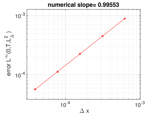
Figure 2: Experimental rate of convergence for cnoidal-wave solution
