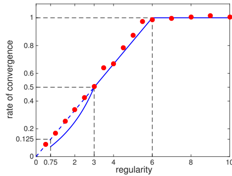
Figure 13: Rates of convergence according to the Sobolev regularity of u_0 . – Rates proved in this paper (solid line) versus experimental rates (dots)
