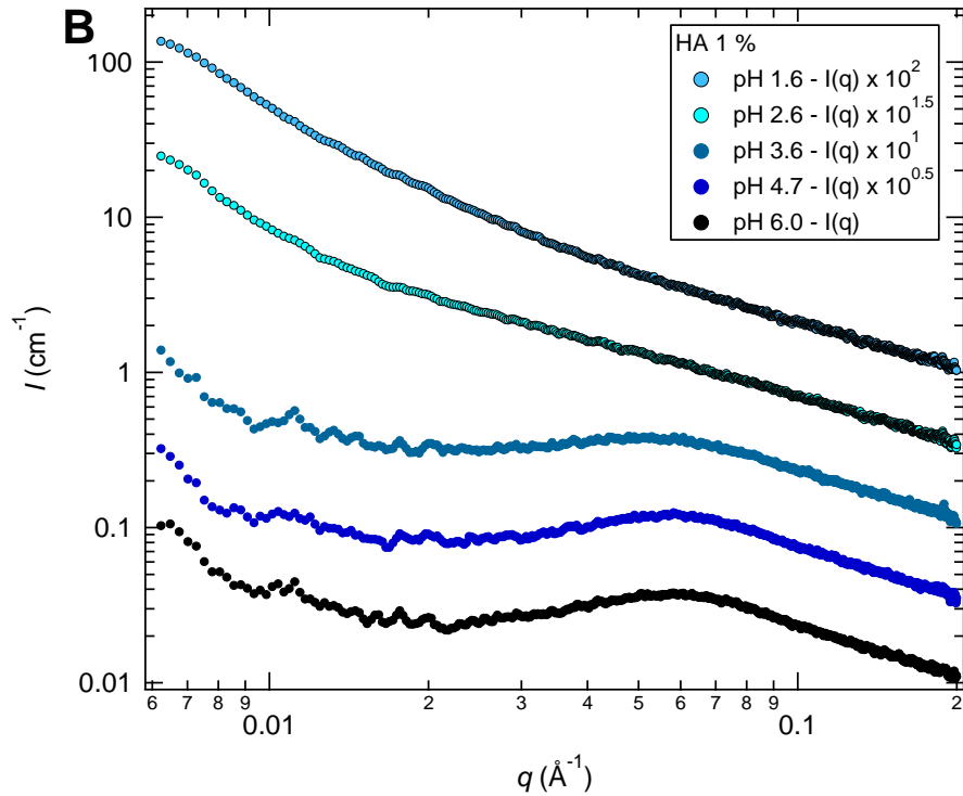
Fig SI-5. [A] Neutron scattering intensity of HA solution at 3 % in deuterium oxide and X-ray scattering intensity of HA solution at 3 % in water. [B] X-ray scattering absolute intensities for Aqueous solutions of HA at 1 % for various pH. For clarity, the intensity at pH 6.0 is has not been modified, the other absolute intensities have been multiplied by successive powers of \sqrt{10} .
