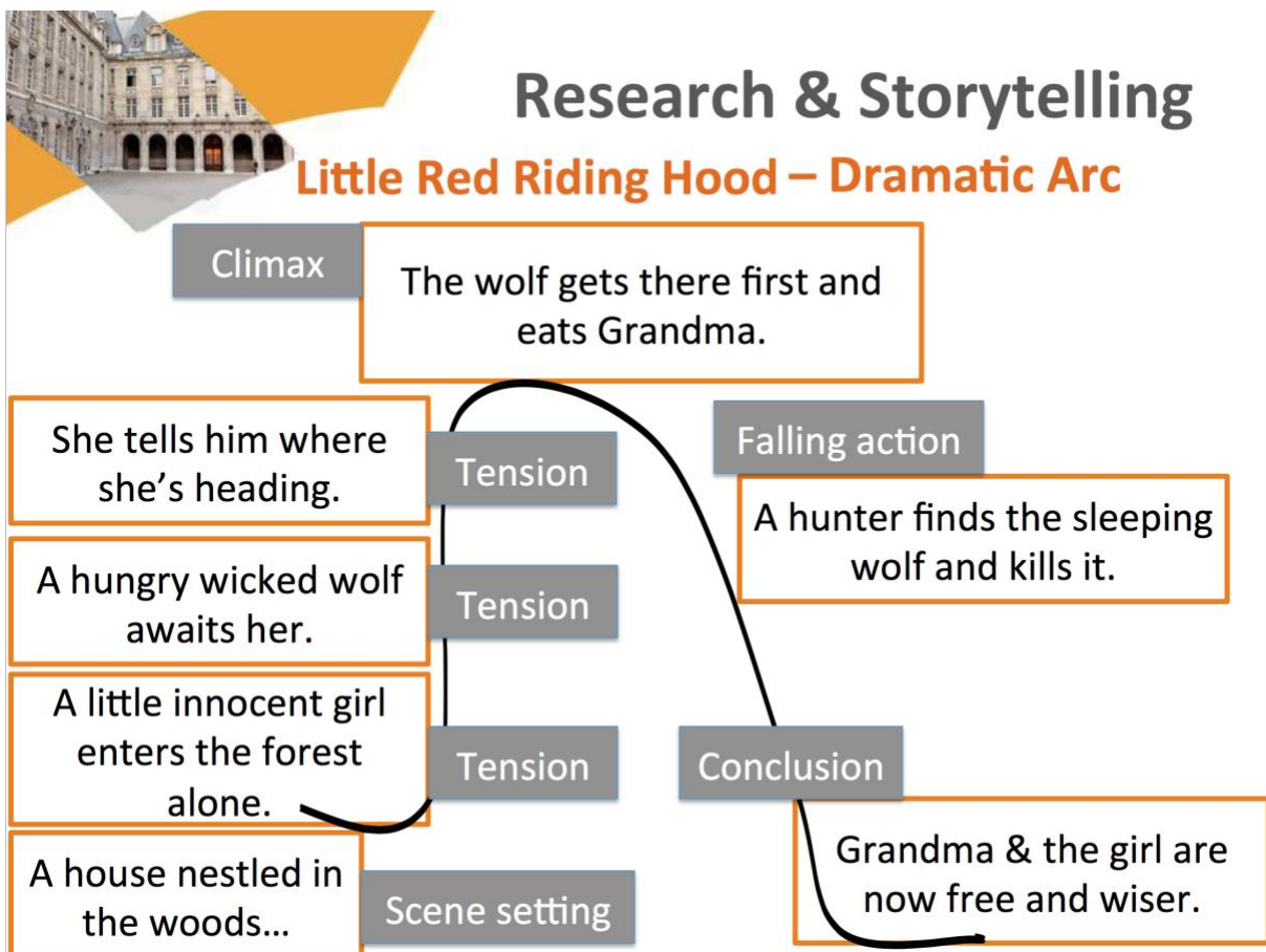
Fig 4. The dramatic arc, adapted from Luna (20013).
