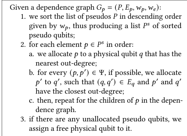
Figure 9. Finding an initial mapping to qubit allocation.
