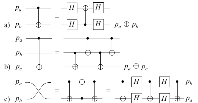
Figure 3. (a) Reversal. (b) Bridge. (c) Swap.
