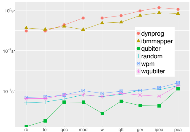
Figure 17. Time, in seconds scaled in \log_{10} (y-axis), spent by the algorithms, when executed with each quantum program.
