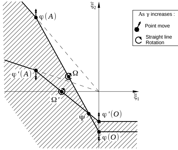
Figure 6: Existence conditions of the equilibrium: comparative statics on \gamma .
