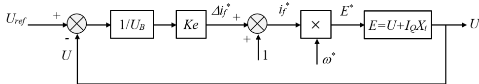
Figure 5. Control block diagram of the VSG excitation regulator.
