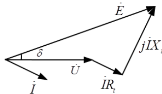
Figure 7. Voltage vector diagram of VSG.
