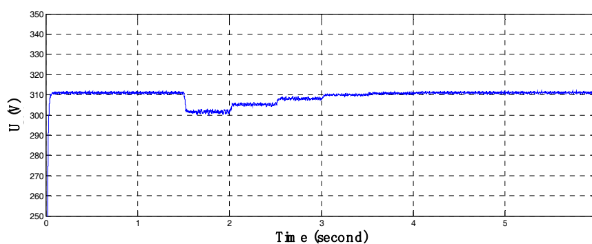
(b) Phase voltage amplitude of Load1
