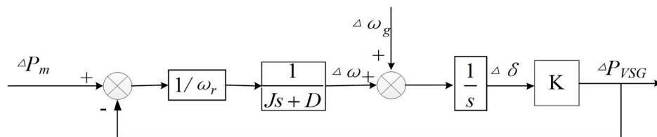
Figure 8. Active power small signal analysis model.
