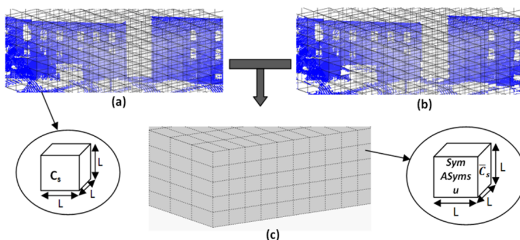
Figure 6. Formulation of 3D evidence grids and similarity map. ((a) and (b)) show the 3D point clouds ( P(n_p) and P(n_p - 1) ) mapped onto an evidence grid of cell size, L^3 , respectively. In (c), the similarity map obtained from the two evidence grids.
