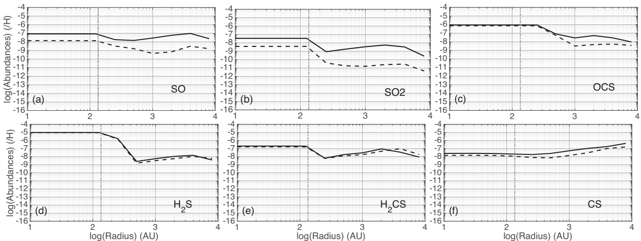
Figure 7. Abundances of SO, SO 2 and OCS (top panel) and H 2 S, H 2 CS and CS (bottom panel), relative to H as a function of the radius to the star IRAS 16293–2422 according to the original structure of Aikawa et al. (2008), for the LEDC (solid line) and EDC (dashed line) pre-collapse compositions. The vertical grey dashed line represents the hot core spatial limit R_{\text{HC}} = 135 au, T > 100 K.
