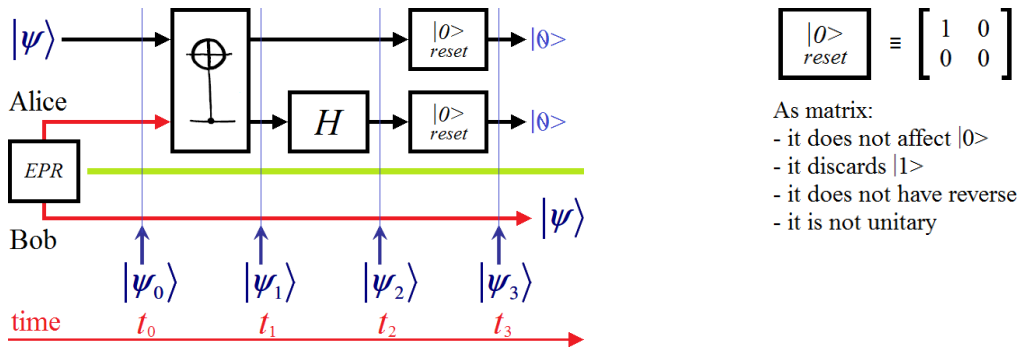
Figure 6.6 Simplified Teleportation protocol using an EPR pair but without classical bits for disambiguation.
