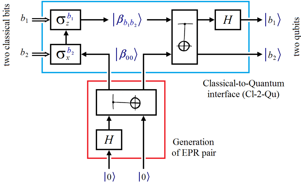
Figure 6.8 Classical-to-Quantum interface.
