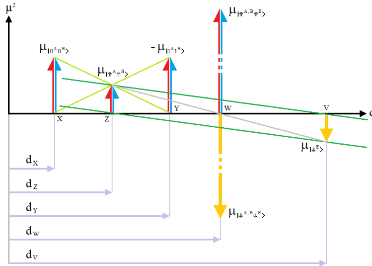
Figure 3.14 Two completely independent spins ( \mu_{|0^{A_0B}} and \mu_{|1^{A_1B}} ) are entangled with a third isolated spin \mu_{|U^E} .
