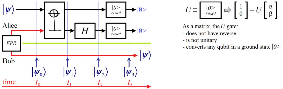
Figure 6.6 Simplified Teleportation protocol using an EPR pair but without classical bits for disambiguation.
