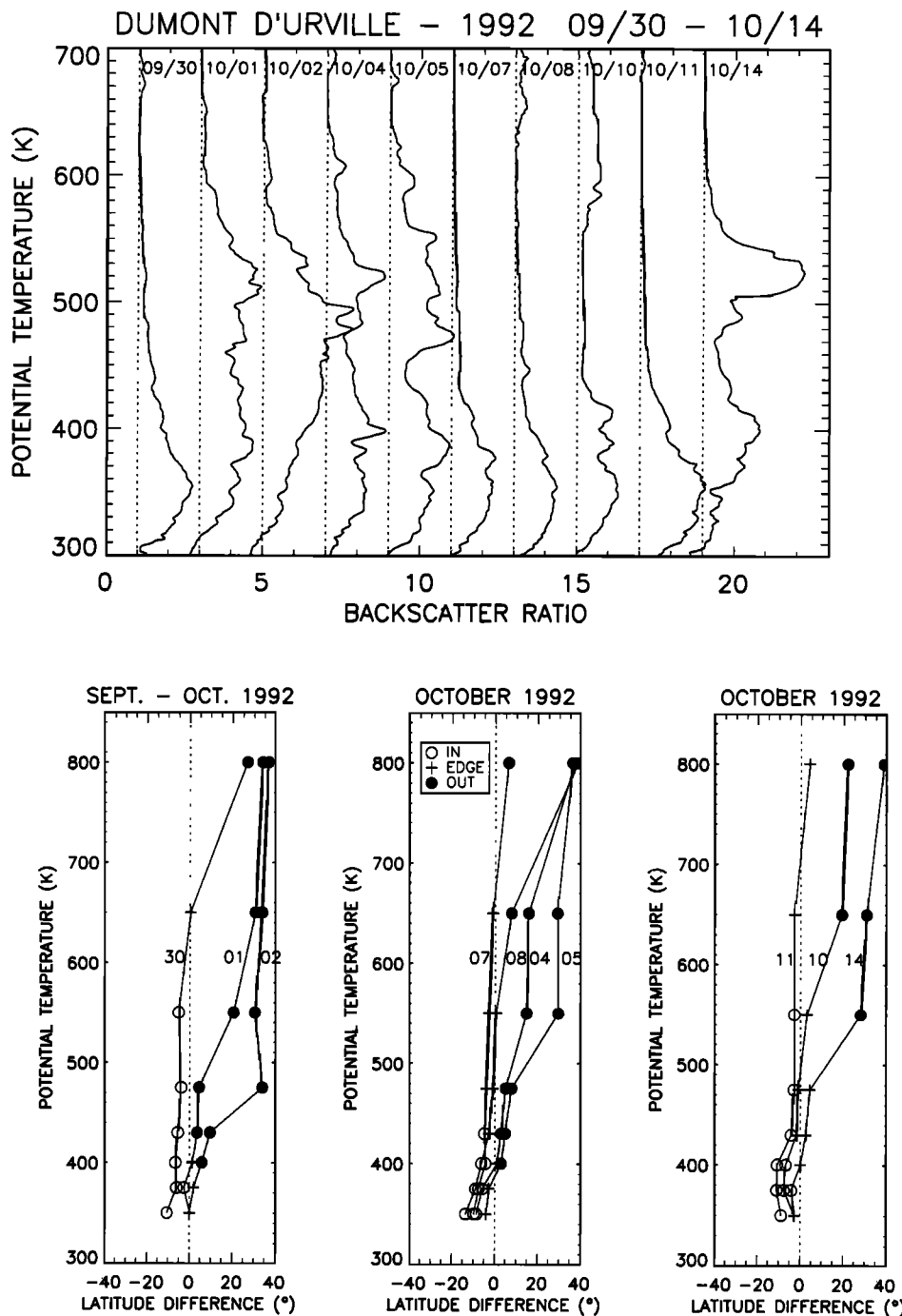
Figure 10. (top) Temporal evolution of the aerosol backscatter ratio profiles from September 30 to October 14, 1992. (bottom) Difference between the equivalent latitude of Dumont d'Urville and the vortex limit as a function of potential temperature for the days when aerosols lidar measurements were obtained. The date of each profile is indicated.
